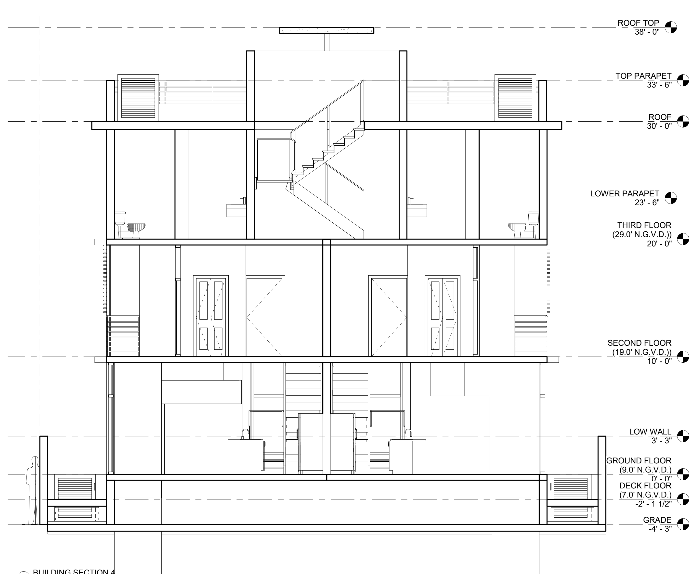
② BUILDING SECTION 4 1/4" = 1'-0"
