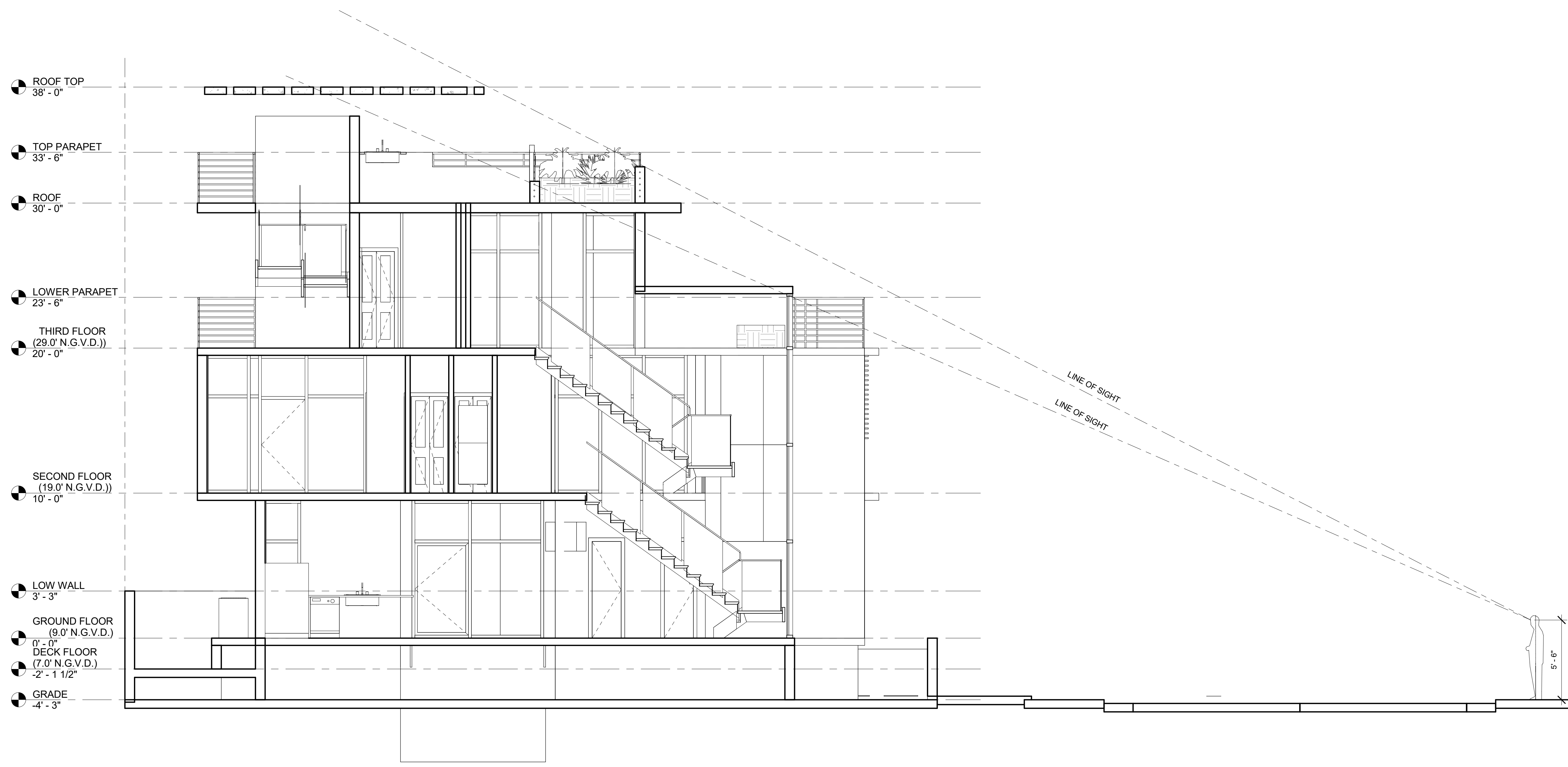
1 BUILDING SECTION 1 1/4" = 1'-0"
