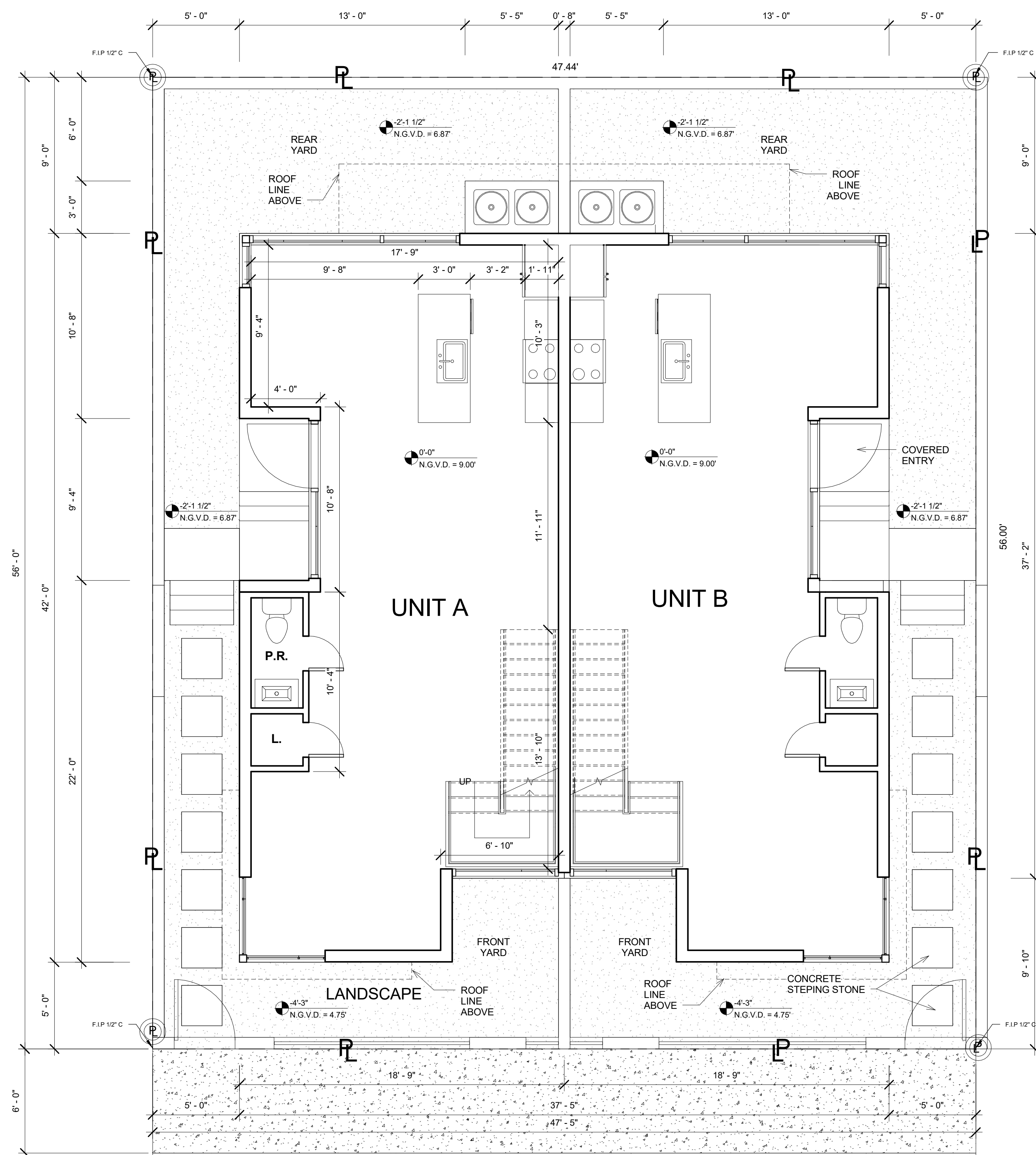
1 GROUND FLOOR (9.0' N.G.V.D.) 1/4" = 1'-0"
