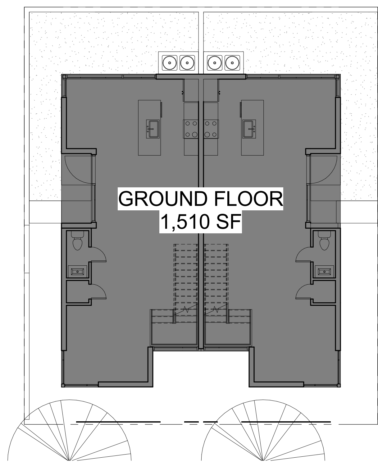
1 FAR GROUND FLOOR 1/8" = 1'-0"
