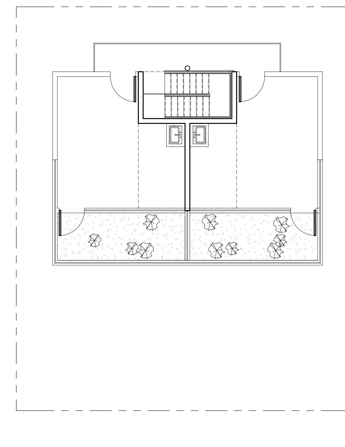
3 FAR ROOF 1/8" = 1'-0"
