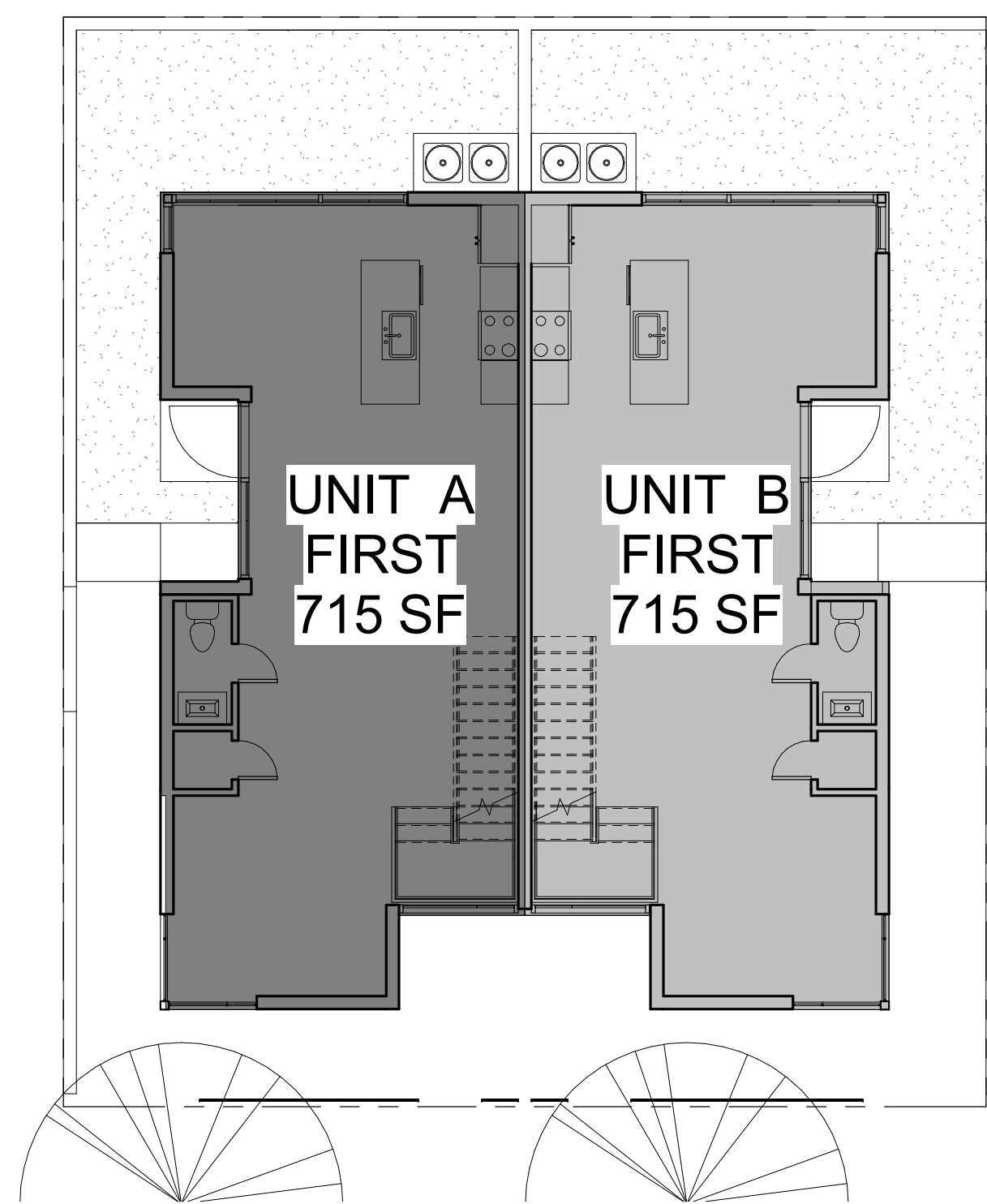
5 UNIT SIZE GROUND 1/8" = 1'-0"
