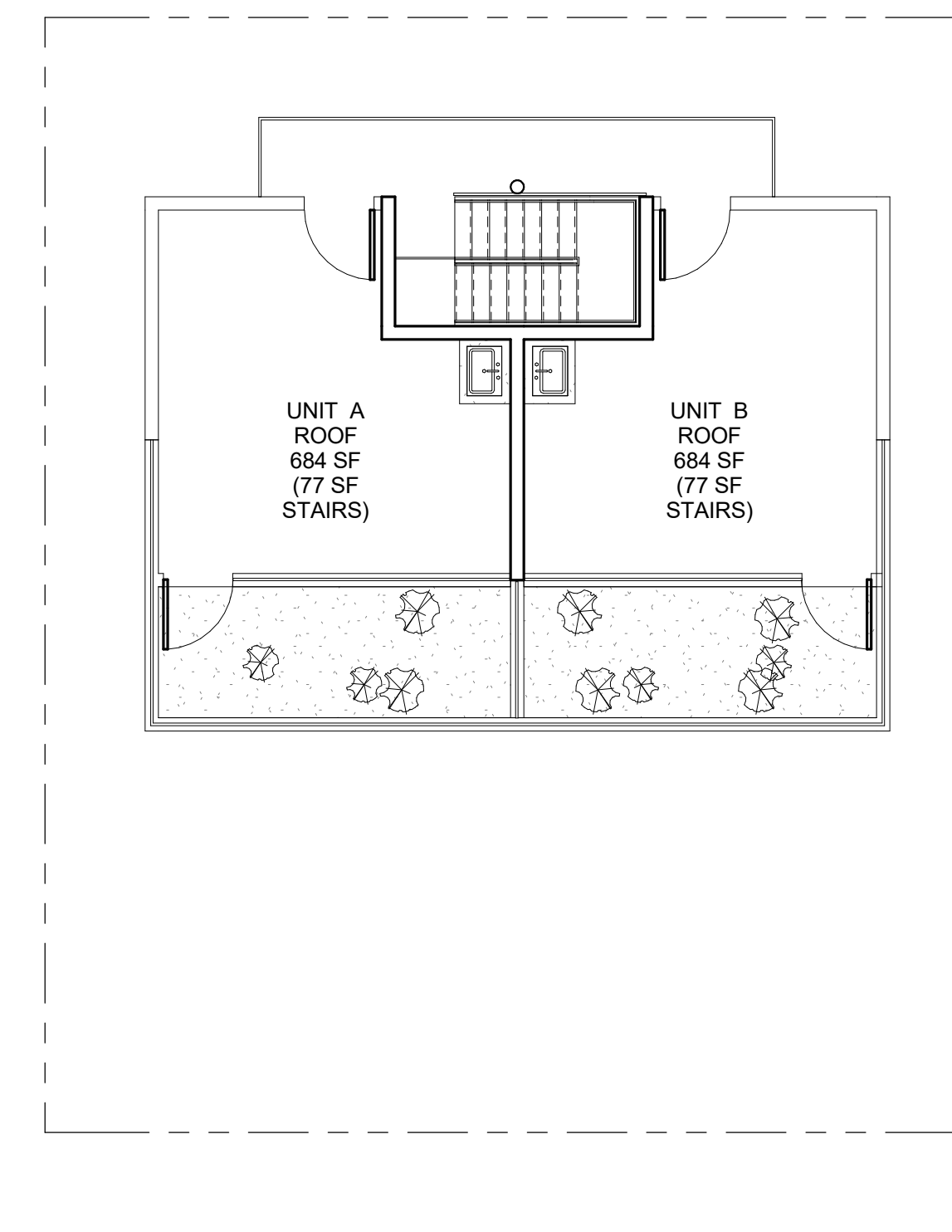
8 UNIT SIZE ROOF 1/8" = 1'-0"
