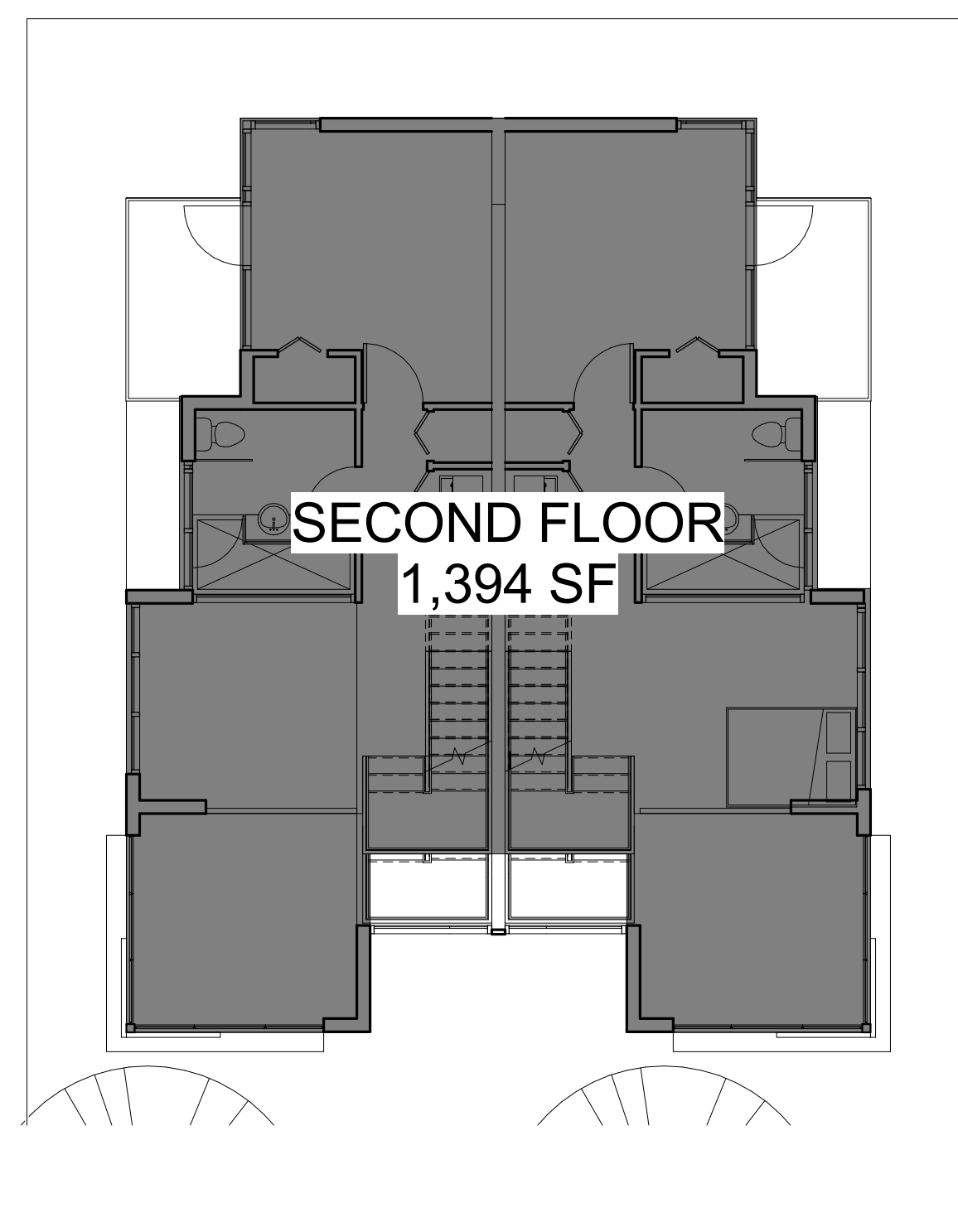
2 FAR SECOND FLOOR 1/8" = 1'-0"
