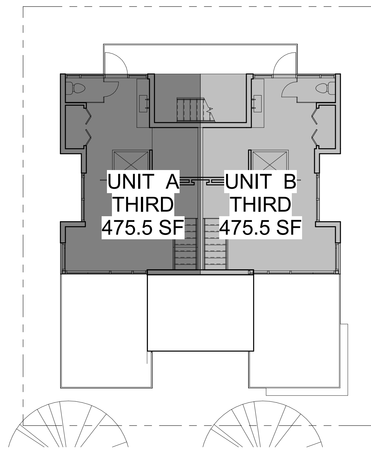
7 UNIT SIZE THIRD 1/8" = 1'-0"
