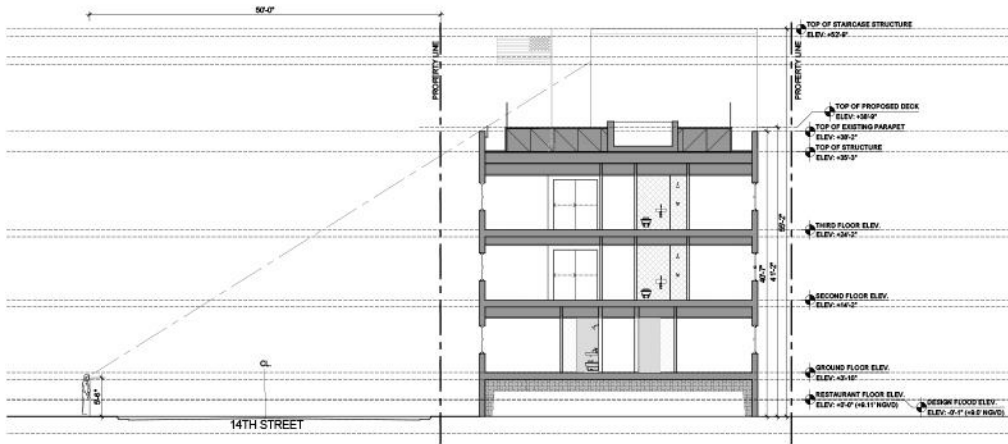
PROPOSED NORTH SECTION
