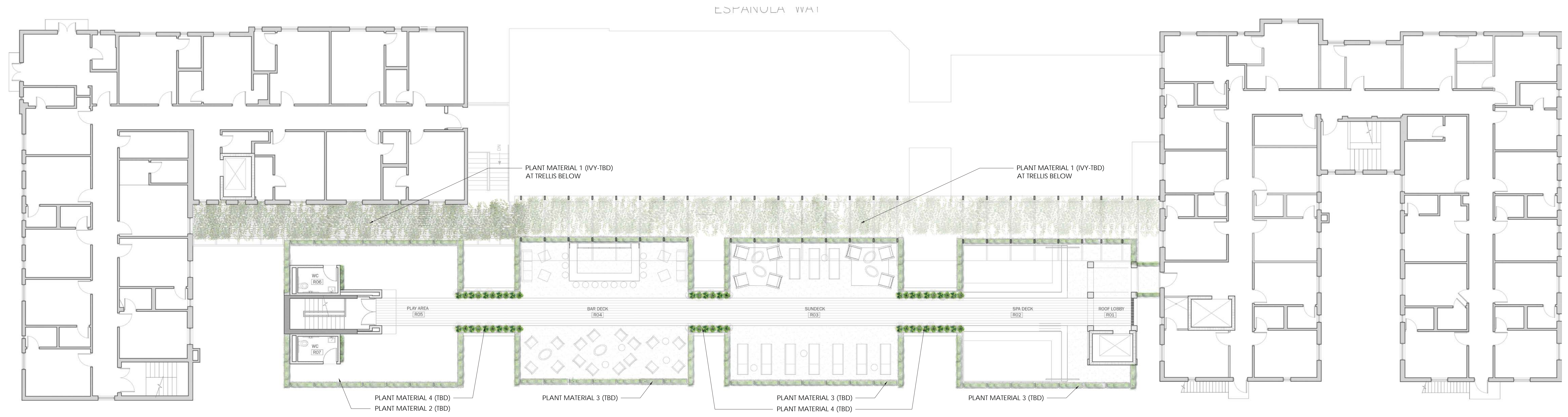
THIRD FLOOR LANDSCAPE PLAN 0 10'-8" 21'-4" 42'-8" SCALE: 3/32" = 1'-0"
