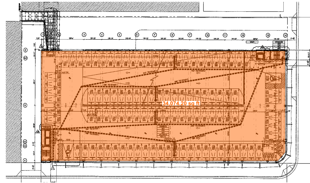
3 LEVEL 03, 04, & 05 PARKING
