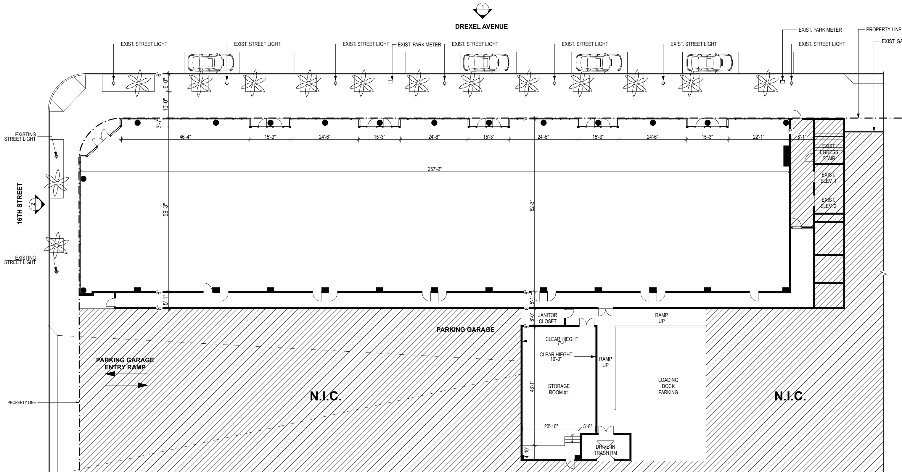
1 EXISTING GROUND LEVEL SCALE: 1" = 20'
