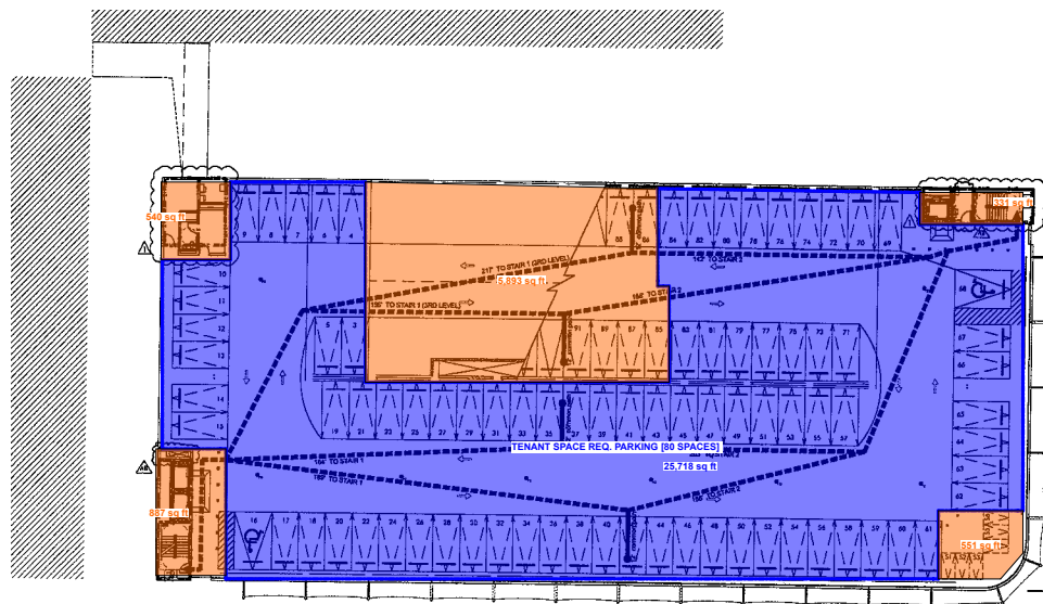
2 LEVEL 02 PARKING
