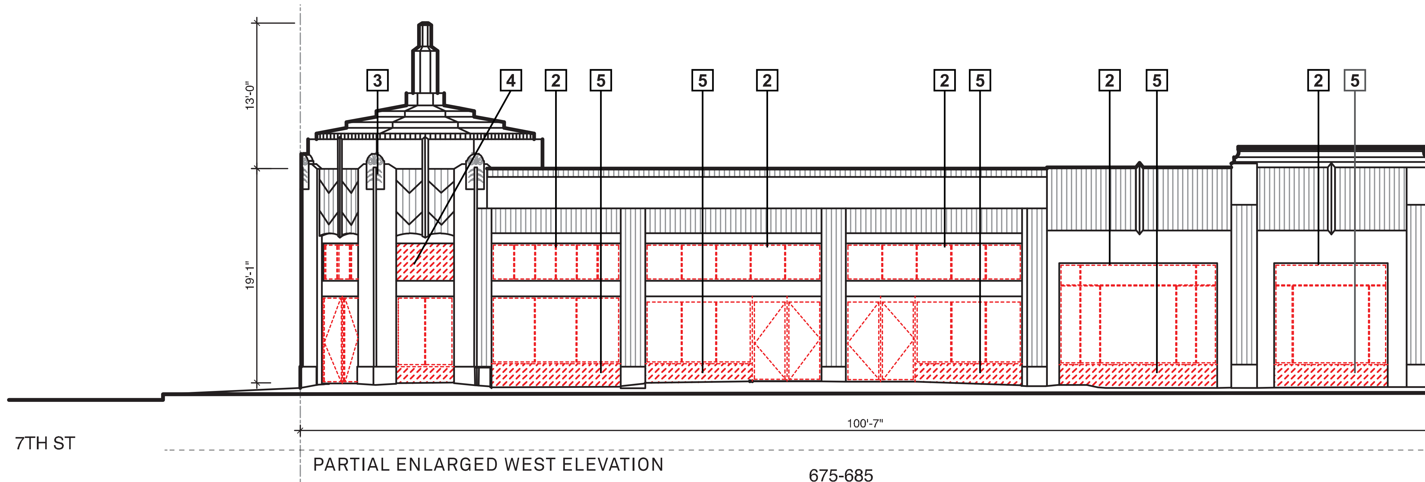
WEST ELEVATION
