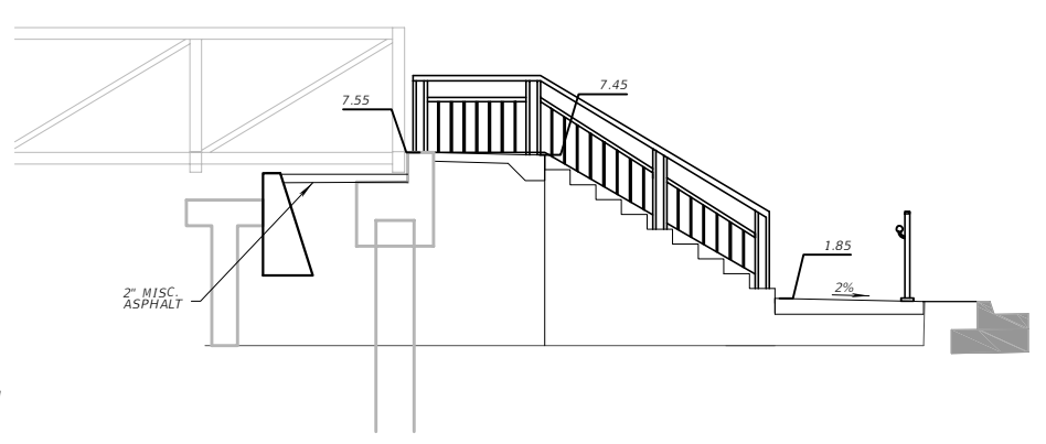
CROSS SECTION B-B
