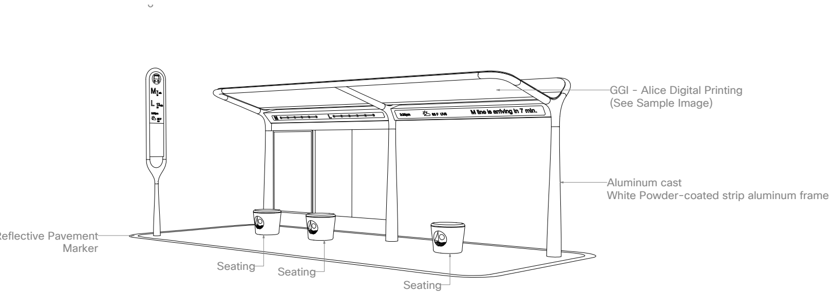
PERSPECTIVE VIEW
