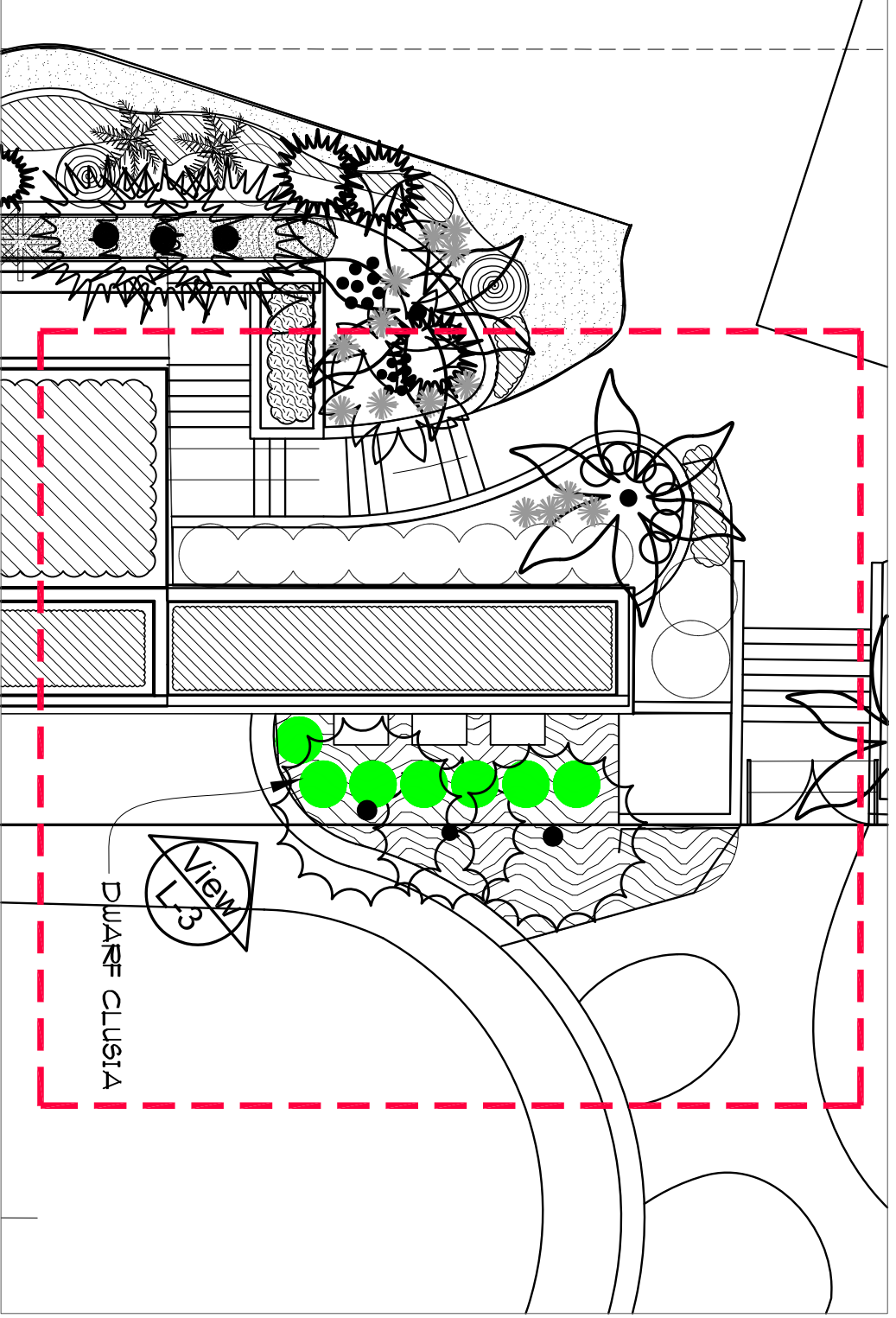
32nd STREET AC SCREEN - CONCEPTUAL LAYOUT PLAN SCALE: 3/32" = 1'-0"
