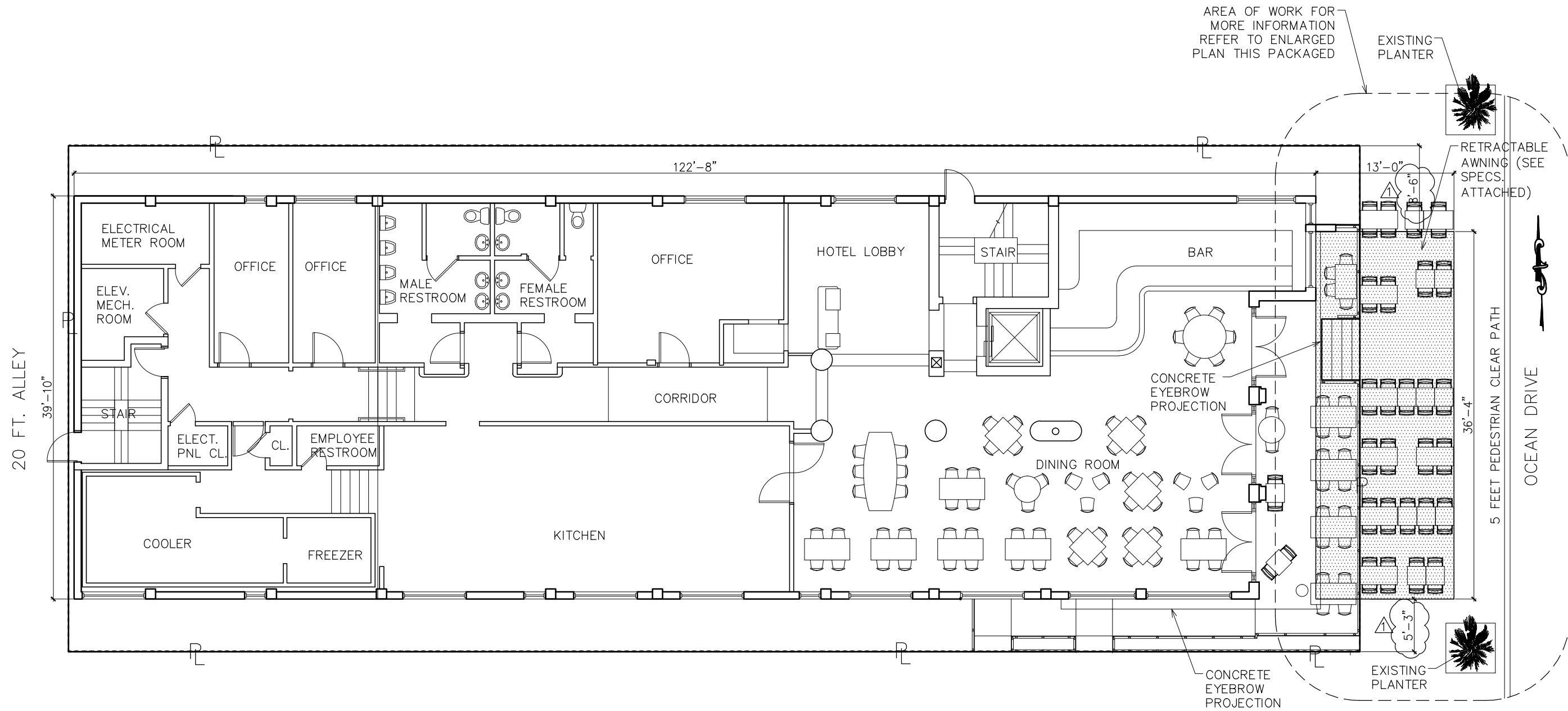
FLOOR PLAN (826 OCEAN DR) SCALE : 3/32" = 1'-0"
