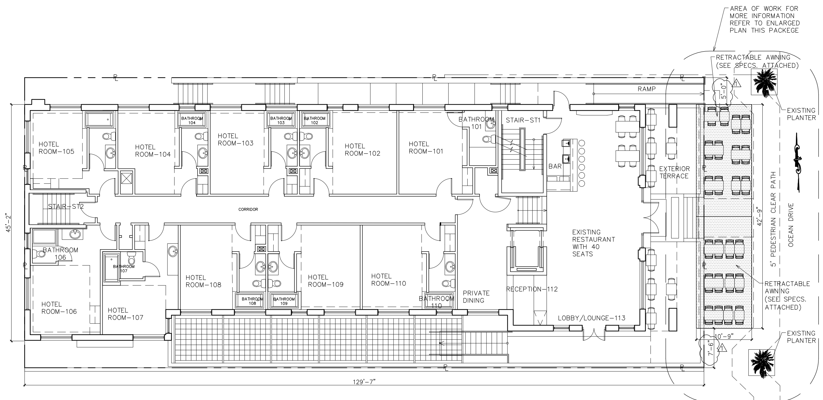
FLOOR PLAN (1244 OCEAN DR) SCALE : 3/32" = 1'-0"
