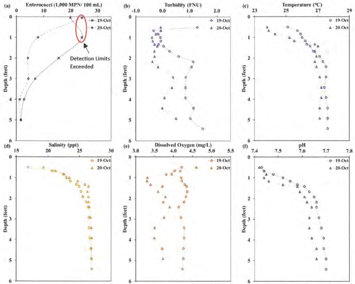
Figure V.15: Measurements versus depth at the KKW. Panel (a) enterococci concentrations; Panel (b) turbidity; Panel (c) temperature; Panel (d) salinity; Panel (e) dissolved oxygen; and Panel (f) pH.
