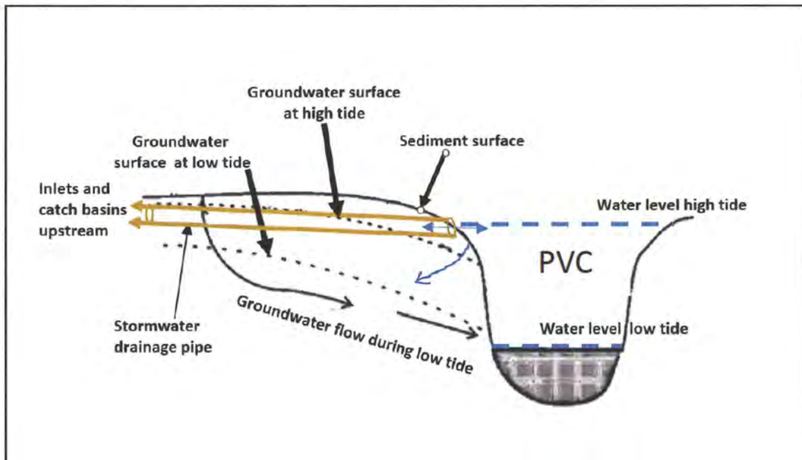
Figure III.6: Conceptual image of groundwater flows to PVC during high and low tide.
