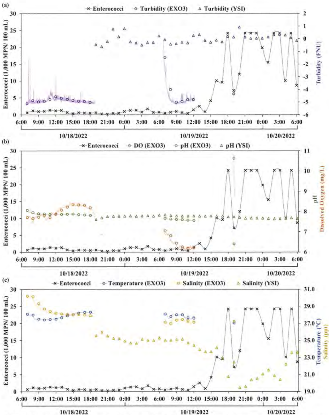
Figure V.14: Enterococci concentration at the KLV during the 48-hour sampling effort with related physical chemical parameters: Panel (a) includes turbidity; Panel (b) includes pH and dissolved oxygen; and Panel (c) includes temperature and salinity.
