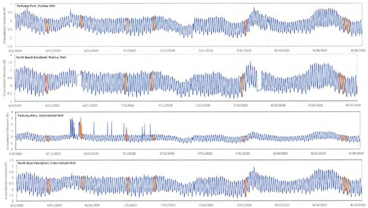
Figure B.3: Time series plot of groundwater data from the Parkview Park and North Beach Bandshell groundwater monitoring well. Dates of heat maps are highlighted for the months June, July and August 2020. The horizontal straight lines correspond to missing data. Groundwater elevations are in NAVD.
