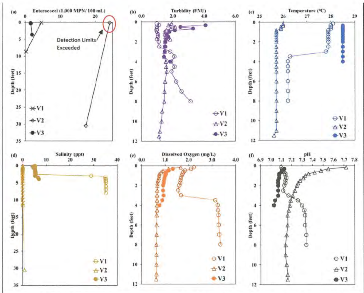
Figure V.17: Vertical drainage wells measurements (V1, V2 and V3) collected on November 14, 2022. Panel (a) enterococci concentration; Panel (b) turbidity; Panel (c) temperature; Panel (d) salinity; Panel (e) dissolved oxygen; and Panel (f) pH.
