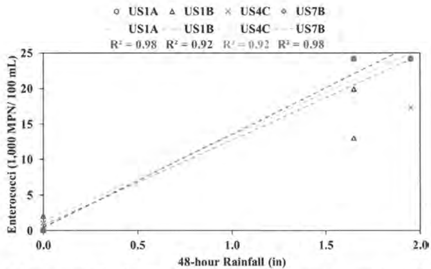
Figure II.8: Linear correlation between enterococci in the upstream samples (US1A, US1B, US4C, and US7B) and 48-hour cumulative precipitation prior to the sampling time based on the Pearson's analysis ( R^2 ).
