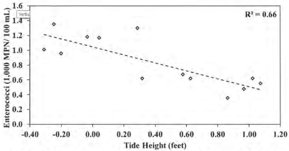
Figure V.12: Linear correlation between the concentration of enterococci and height of tide (water level) from 7:00 to 19:00 on Oct. 18, 2022.
