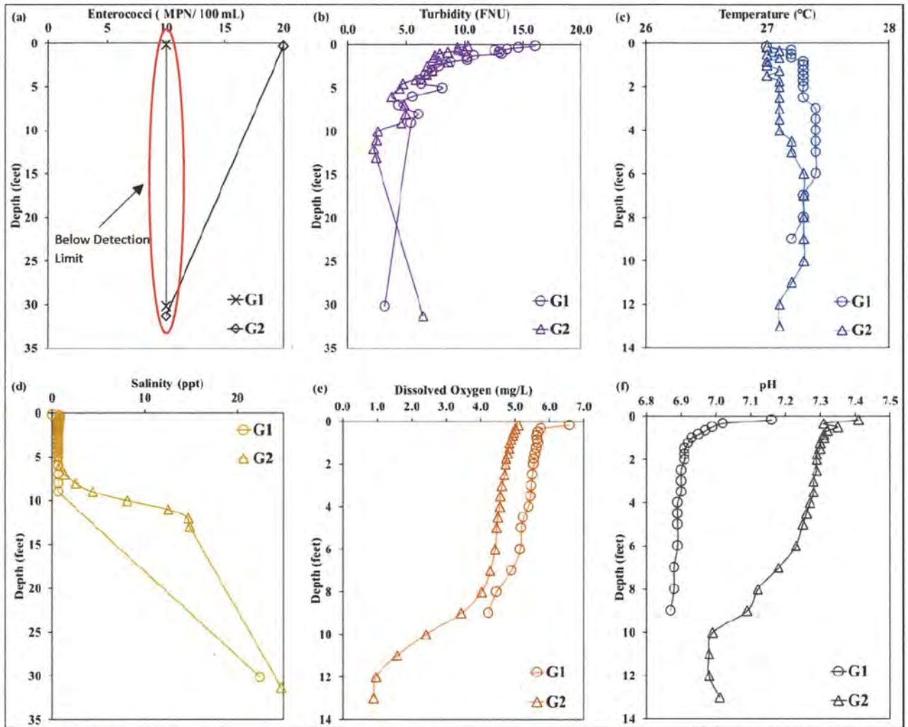
Figure V.18: Groundwater measurements at stations G1 (Bandshell) and G2 (Parkview Island) collected on November 14, 2022. Panel (a) enterococci concentration; Panel (b) turbidity; Panel (c) temperature; Panel (d) salinity; Panel (e) dissolved oxygen; and Panel (f) pH.
