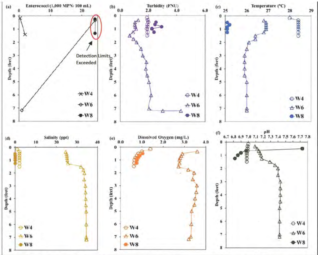
Figure V.16: Catch basin measurements (W4, W6 and W8) collected on November 14, 2022. Panel (a) enterococci concentration; Panel (b) turbidity; Panel (c) temperature; Panel (d) salinity; Panel (e) dissolved oxygen; and Panel (f) pH.
