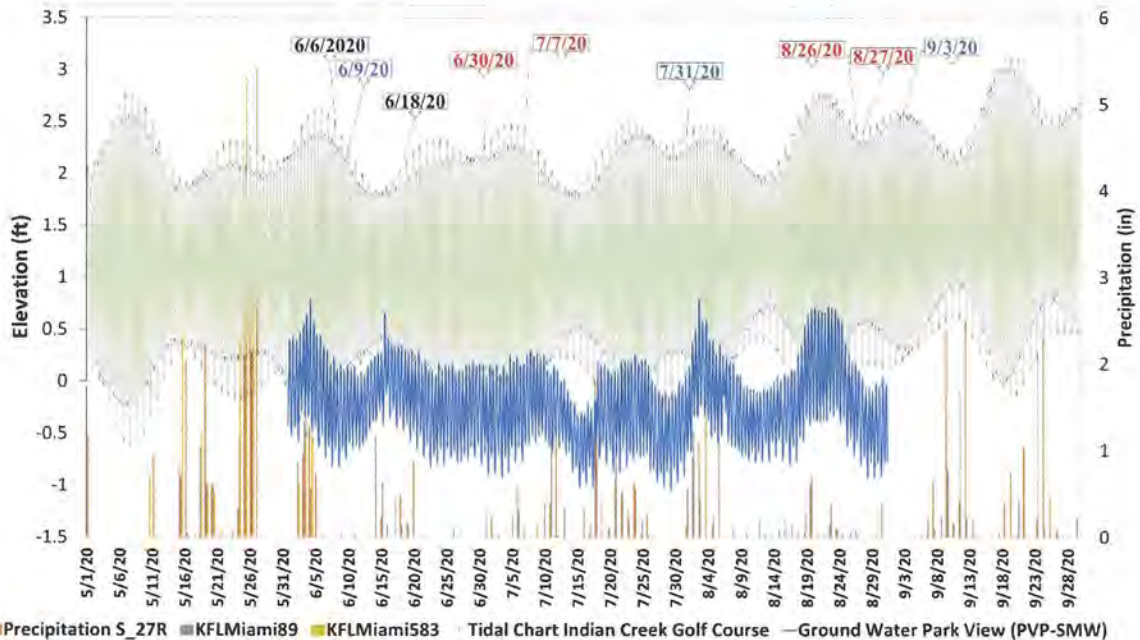
Figure II.3: Time series plot of rainfall, tides and groundwater superimposed on dates and peak enterococci levels measured in catch basins. Elevation corresponds to NAVD.
