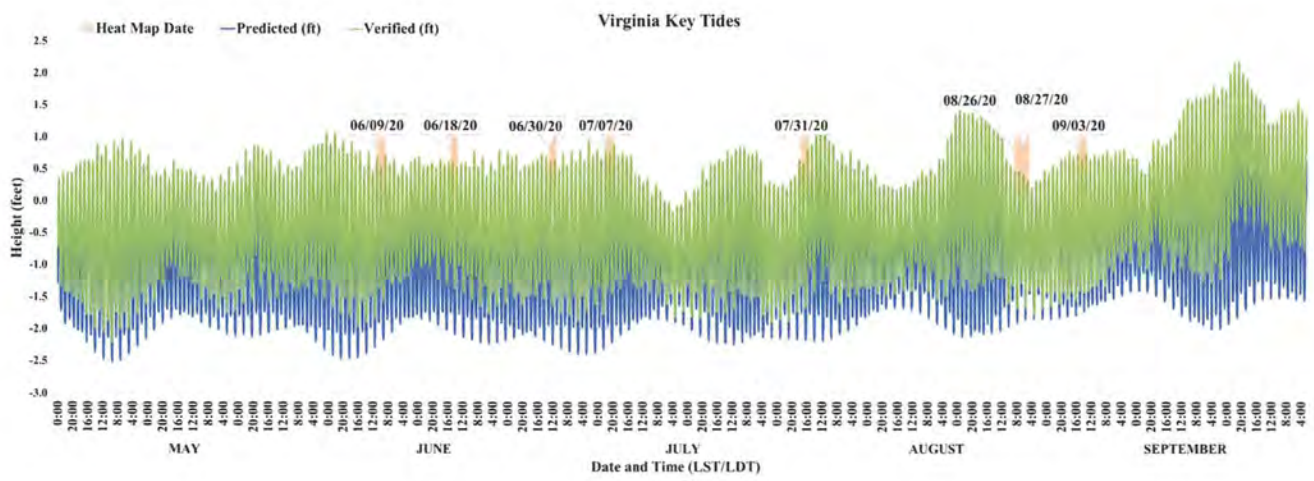
Figure B.4: Virginia Key predicted and verified tides, dates from Heat Maps with FIB peaks. Heights are referenced to NAVD.
