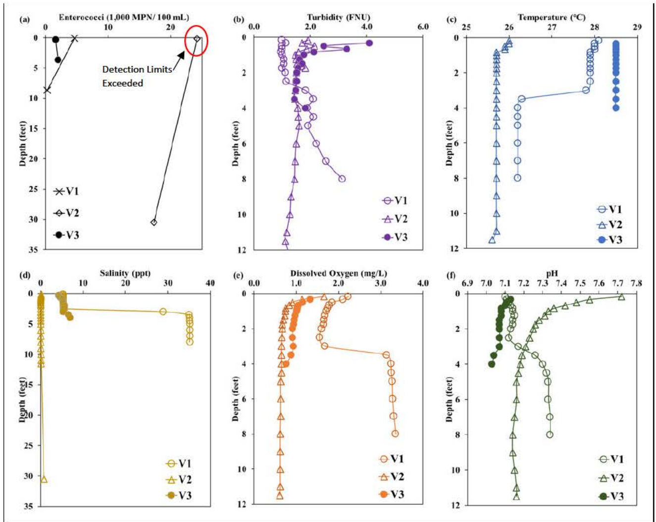
Figure V.17: Vertical drainage wells measurements (V1, V2 and V3) collected on November 14, 2022. Panel (a) enterococci concentration; Panel (b) turbidity; Panel (c) temperature; Panel (d) salinity; Panel (e) dissolved oxygen; and Panel (f) pH.
