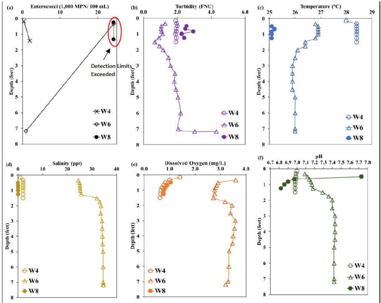
Figure V.16: Catch basin measurements (W4, W6 and W8) collected on November 14, 2022. Panel (a) enterococci concentration; Panel (b) turbidity; Panel (c) temperature; Panel (d) salinity; Panel (e) dissolved oxygen; and Panel (f) pH.
