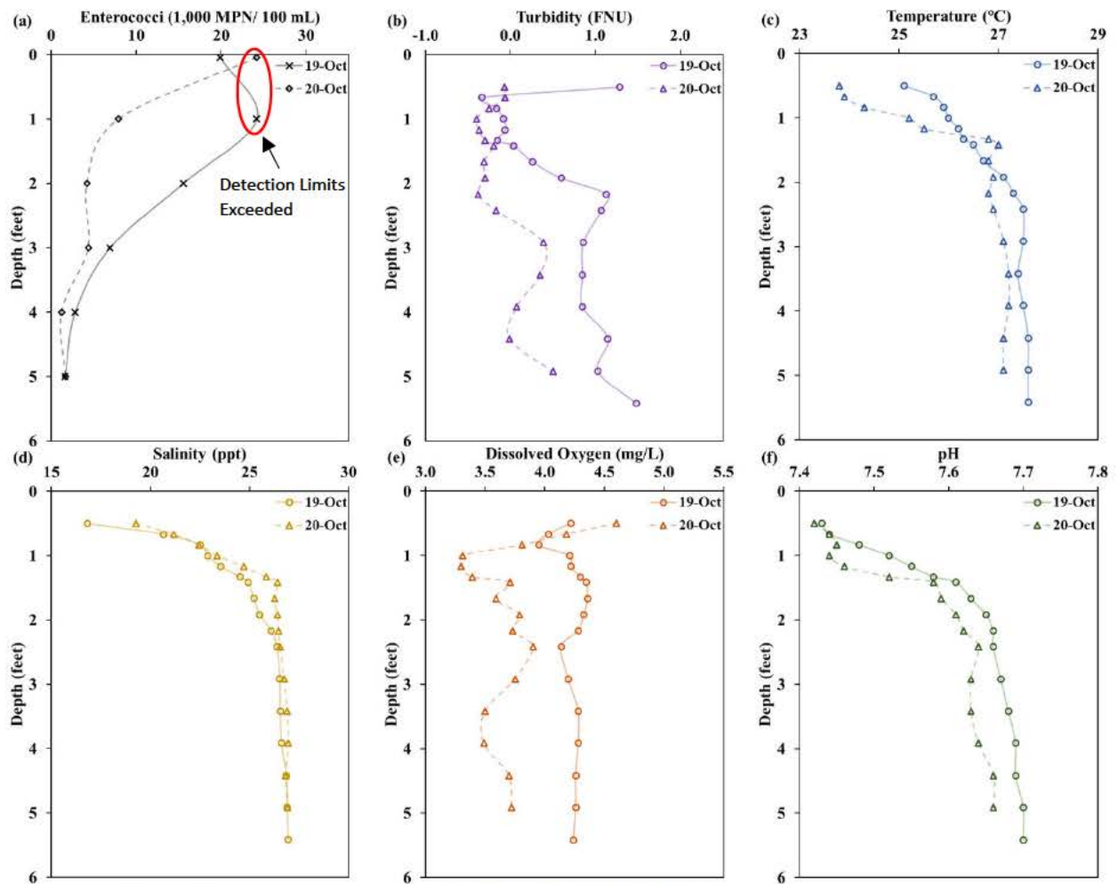
Figure V.15: Measurements versus depth at the KLW. Panel (a) enterococci concentrations; Panel (b) turbidity; Panel (c) temperature; Panel (d) salinity; Panel (e) dissolved oxygen; and Panel (f) pH.
