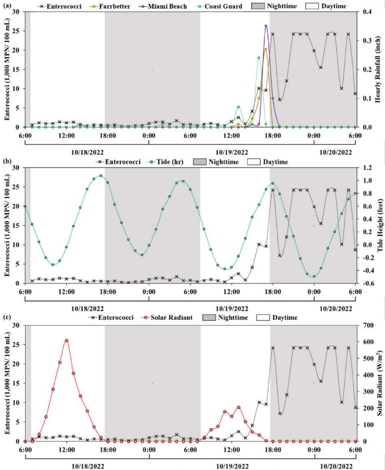
Figure V.11: Enterococci concentration at the K LW during the 48-hour sampling effort along with: Panel (a) hourly rainfall from three closest weather stations; Panel (b) tidal height; and Panel (c) solar radiation. White and grey background indicated daytime and nighttime during the sampling, respectively.
