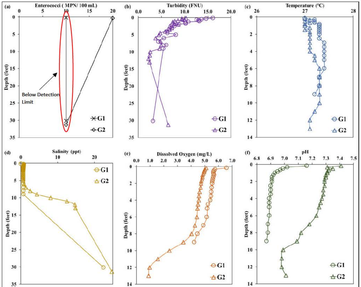
Figure V.18: Groundwater measurements at stations G1 (Bandshell) and G2 (Parkview Island) collected on November 14, 2022. Panel (a) enterococci concentration; Panel (b) turbidity; Panel (c) temperature; Panel (d) salinity; Panel (e) dissolved oxygen; and Panel (f) pH.
