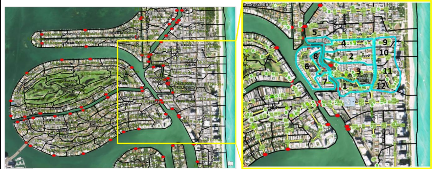
Figure III.1: Stormwater catchment area for PVC shown by heavy blue lines on right panel. Locations of stormwater outfalls are shown by red ovals. This map does not show private outfalls. Total catchment area (catchments 1 to 8 and partial areas for 9 to 12) that discharges stormwater to the PVC is approximately 329,000 m 2 .
