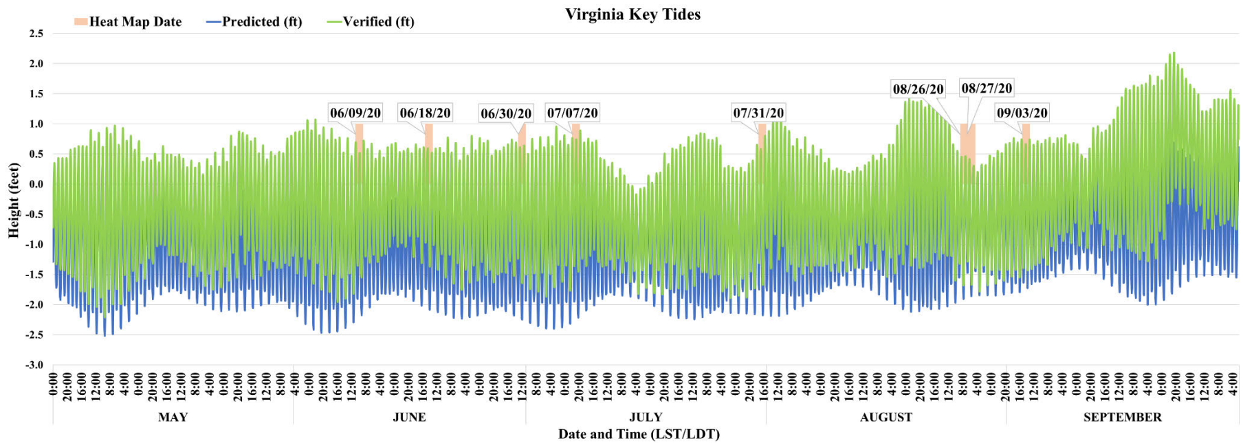
Figure B.4: Virginia Key predicted and verified tides, dates from Heat Maps with FIB peaks. Heights are referenced to NAVD.
