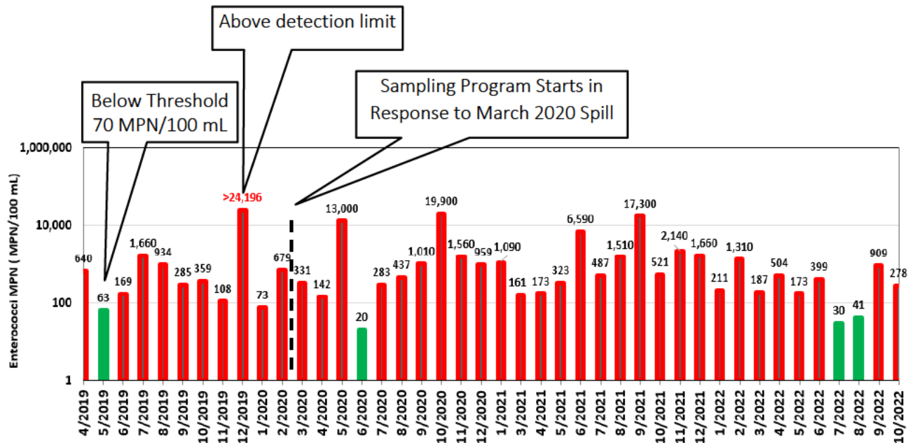
Figure II.1: Results from Monthly Enterococci Measurements at PVC from 4/2019 to 10/2022. Green bars correspond to data points within the 70 MPN/100 mL recommended recreational level whereas red bars correspond to data points which exceed this level. Note the data are plotted on a logarithmic scale due to the wide range of measurements.
