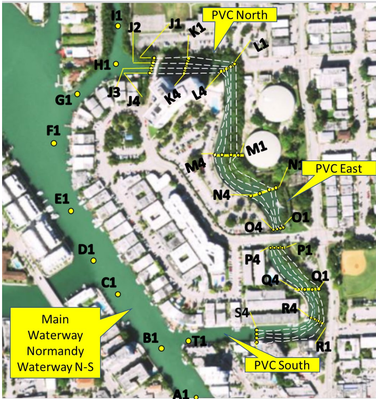
Figure V.2: Map showing transects with sampling locations for intense spatial sampling activity conducted on August 9 th and September 16 th . Red points show the location of the stormwater outfalls, green lines show the location of the stormwater mains, orange line on the northeast bend of the canal shows the location of the siphon, brown lines show the location of the sanitary sewer system force and gravity mains.
