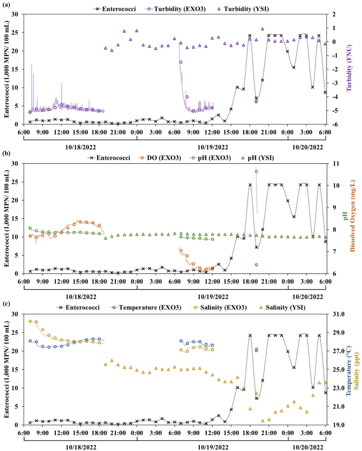
Figure V.14: Enterococci concentration at the K LW during the 48-hour sampling effort with related physical chemical parameters: Panel (a) includes turbidity; Panel (b) includes pH and dissolved oxygen; and Panel (c) includes temperature and salinity.
