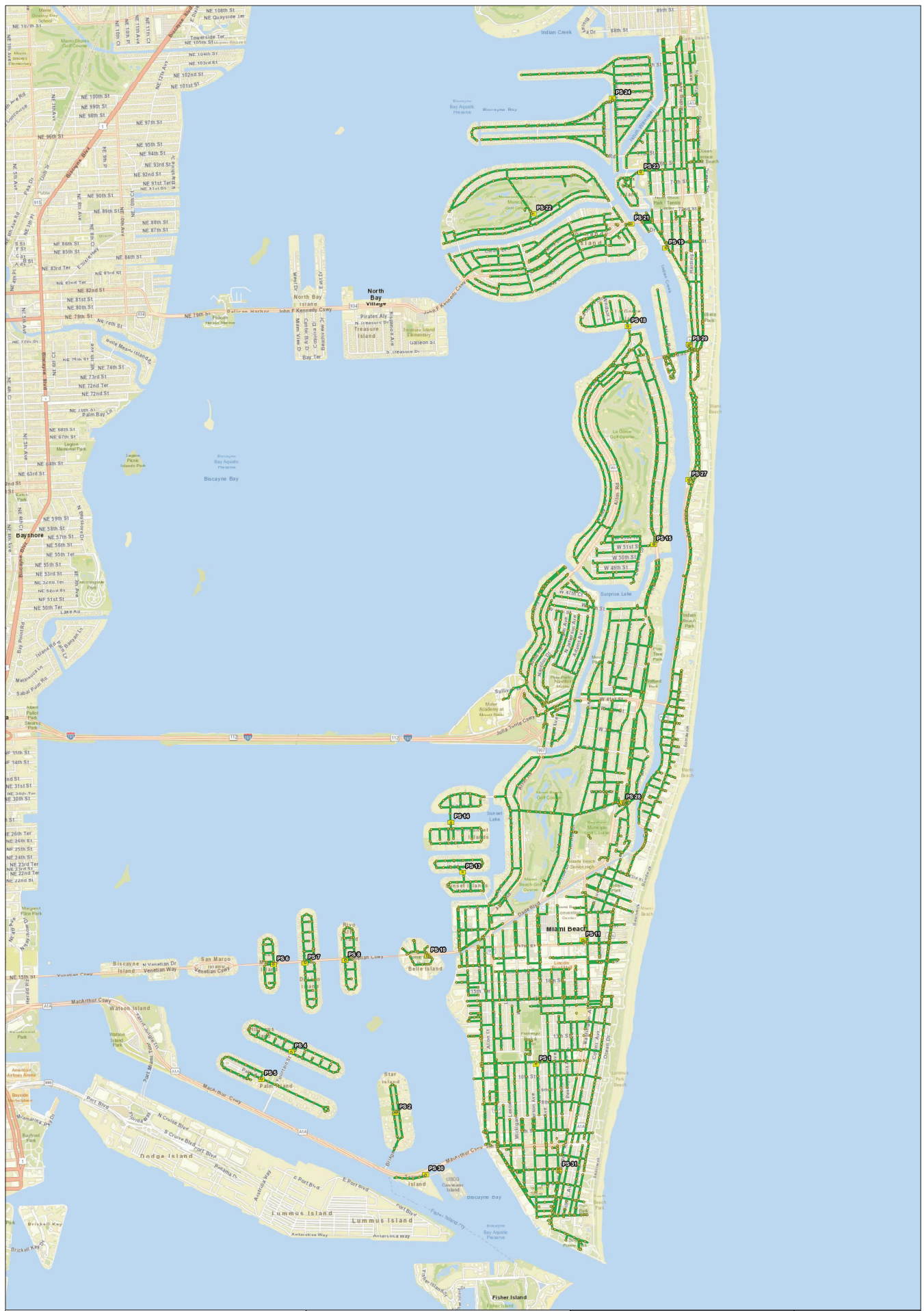
Figure 1-1: Sewer Network Overview
