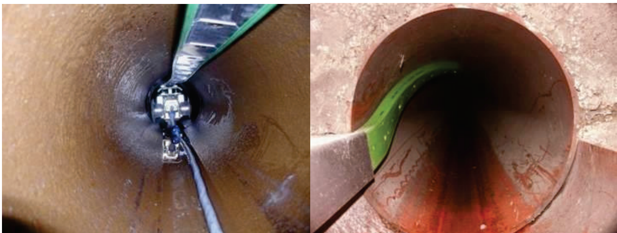
Figure 2-2: CableRunner technology installed in a non-accessible sewer of diameter less than 80 cm (30 in).
