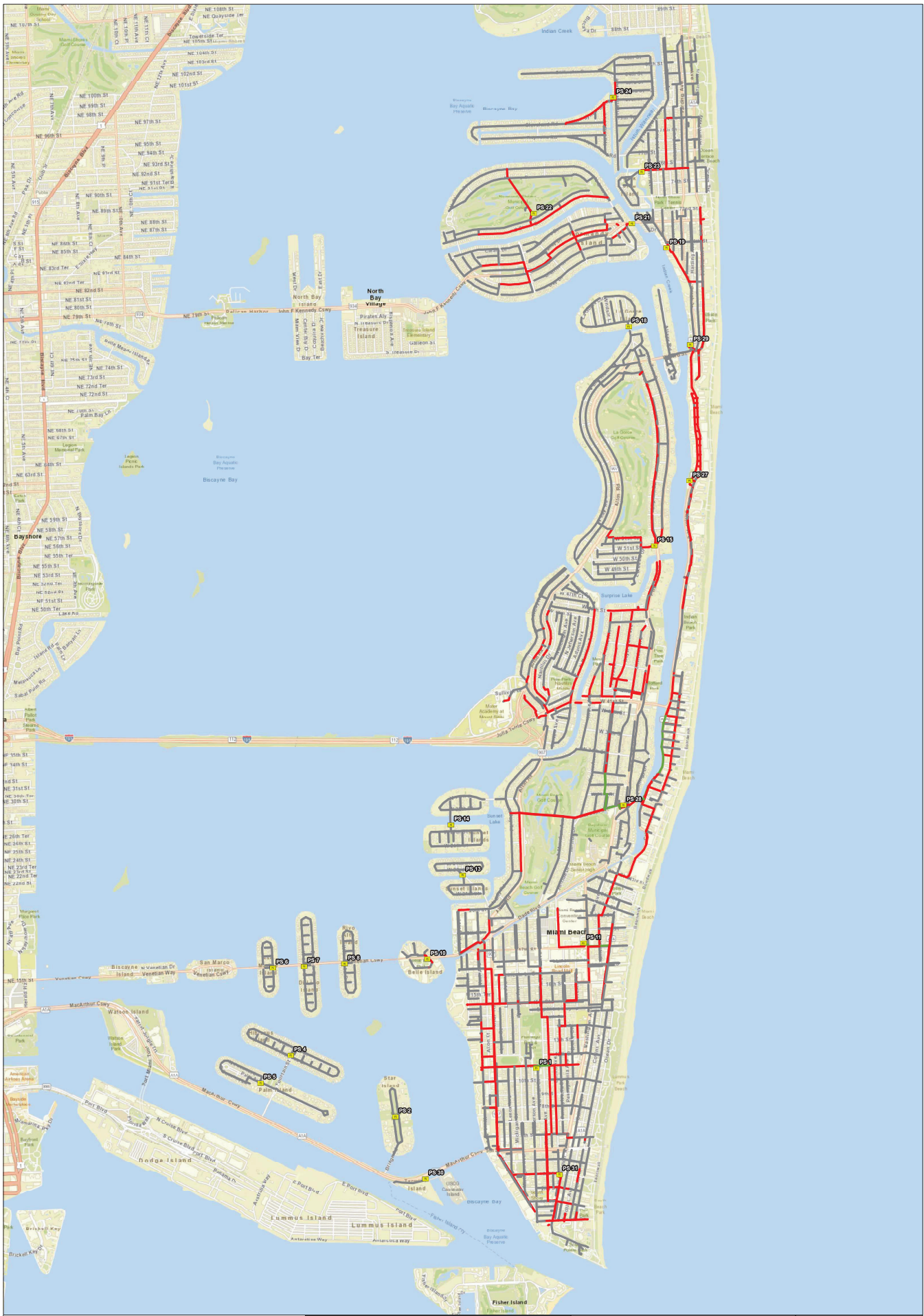
Figure 3-1: Gravity Main Diameter Distribution
