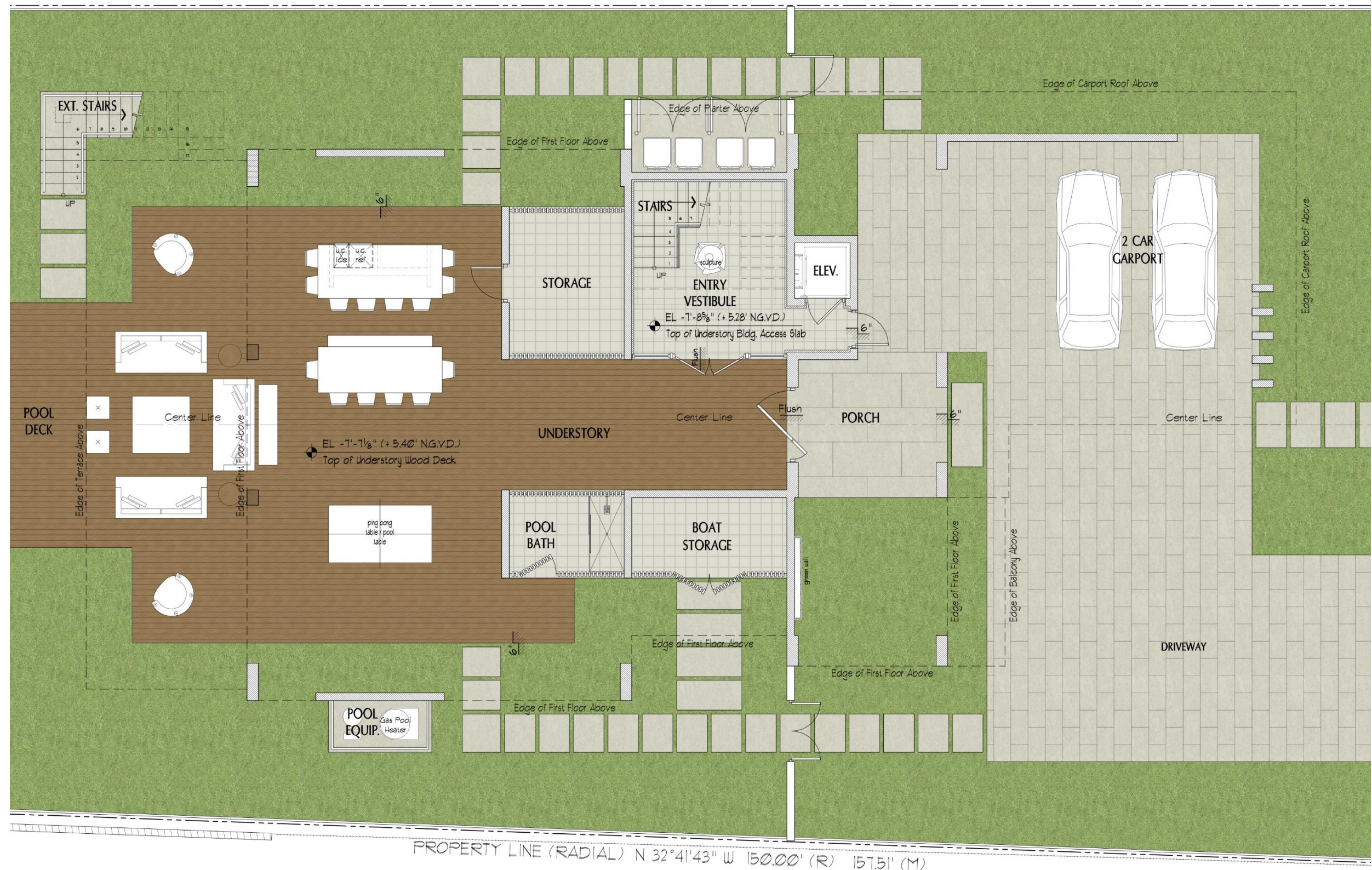
Understory Floor Plan
