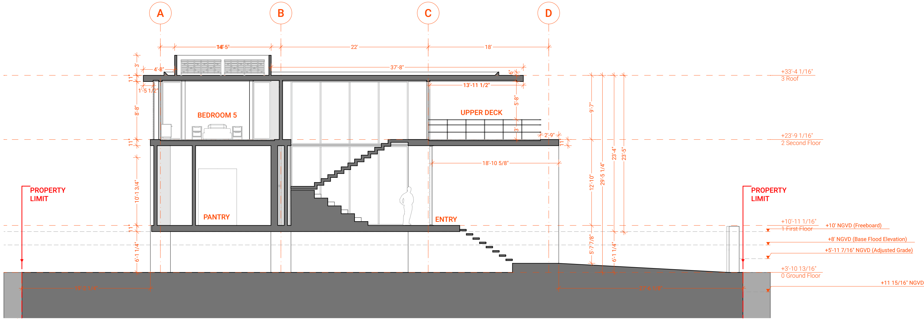
S-01 Cross Section 1:130
