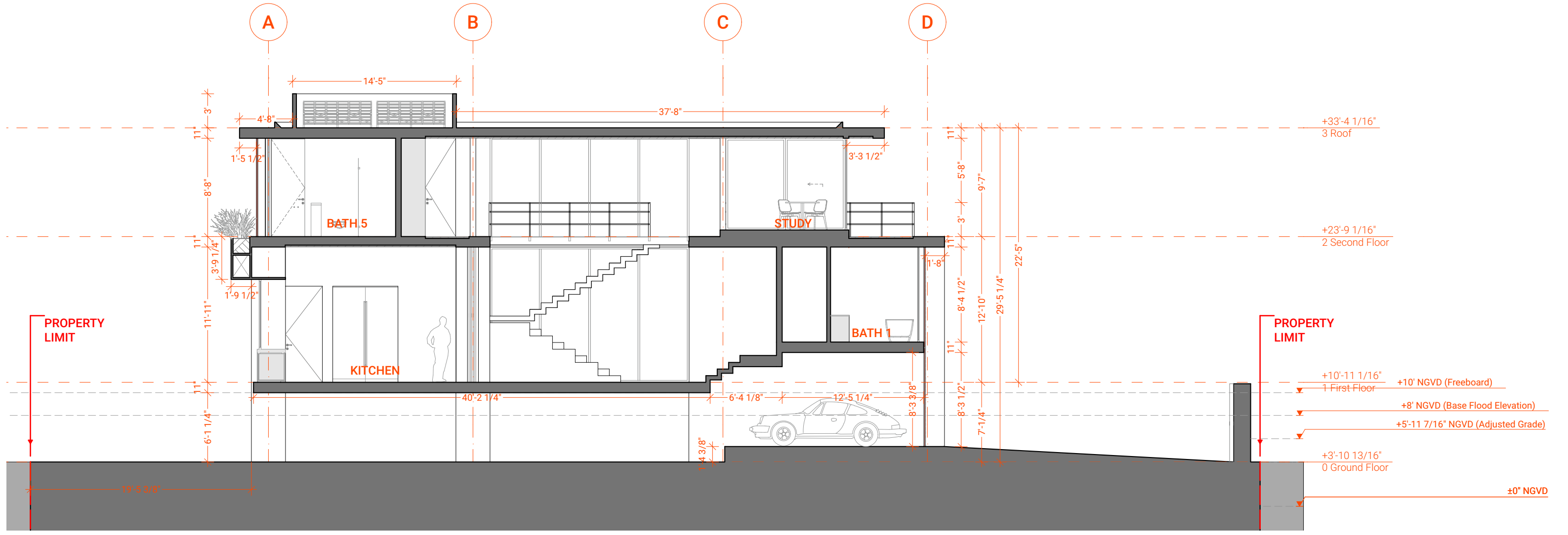
S-02 Cross Section 1:130
