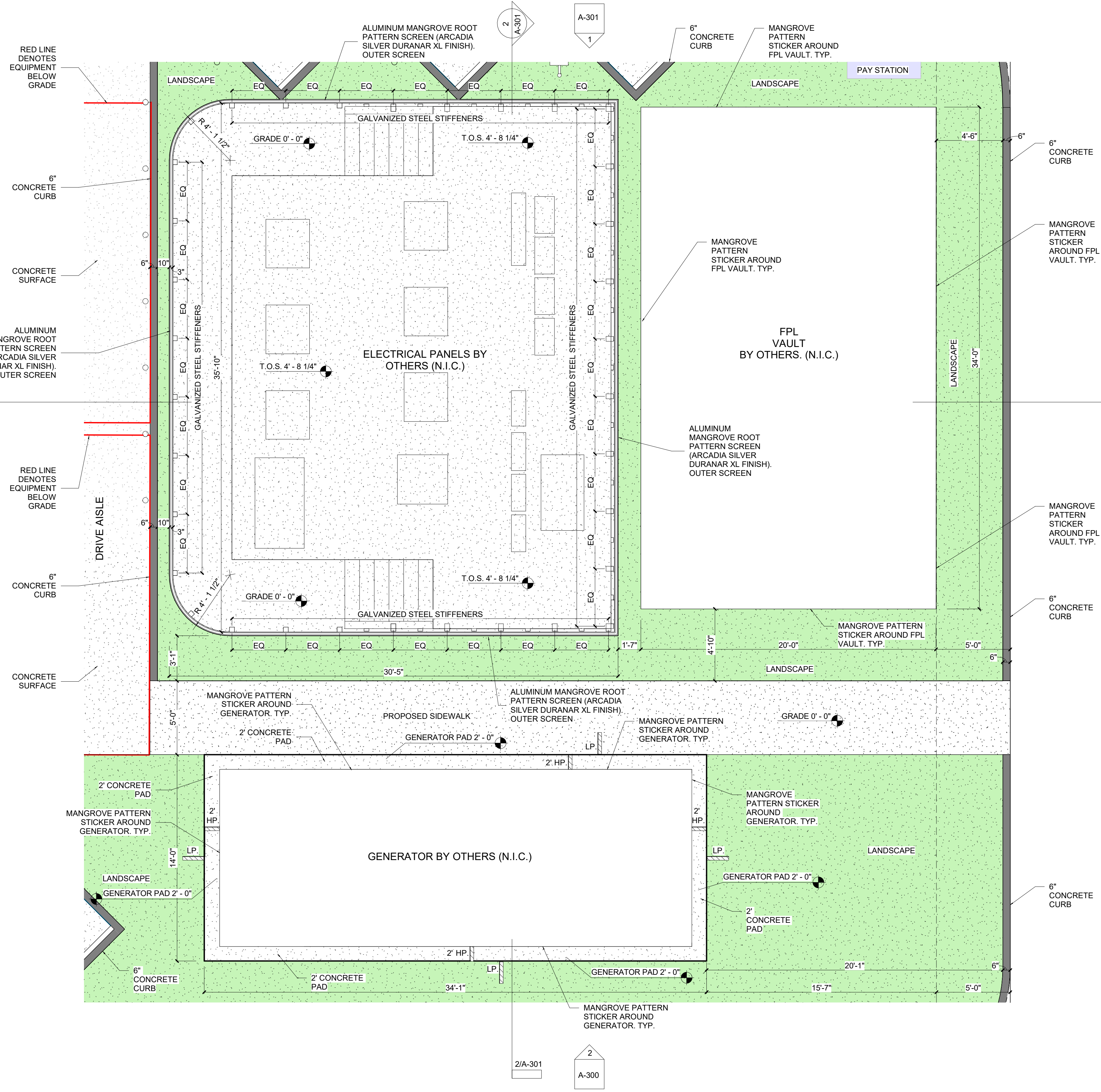
① ENLARGED ELECTRICAL AREA 1/4" = 1'-0"
