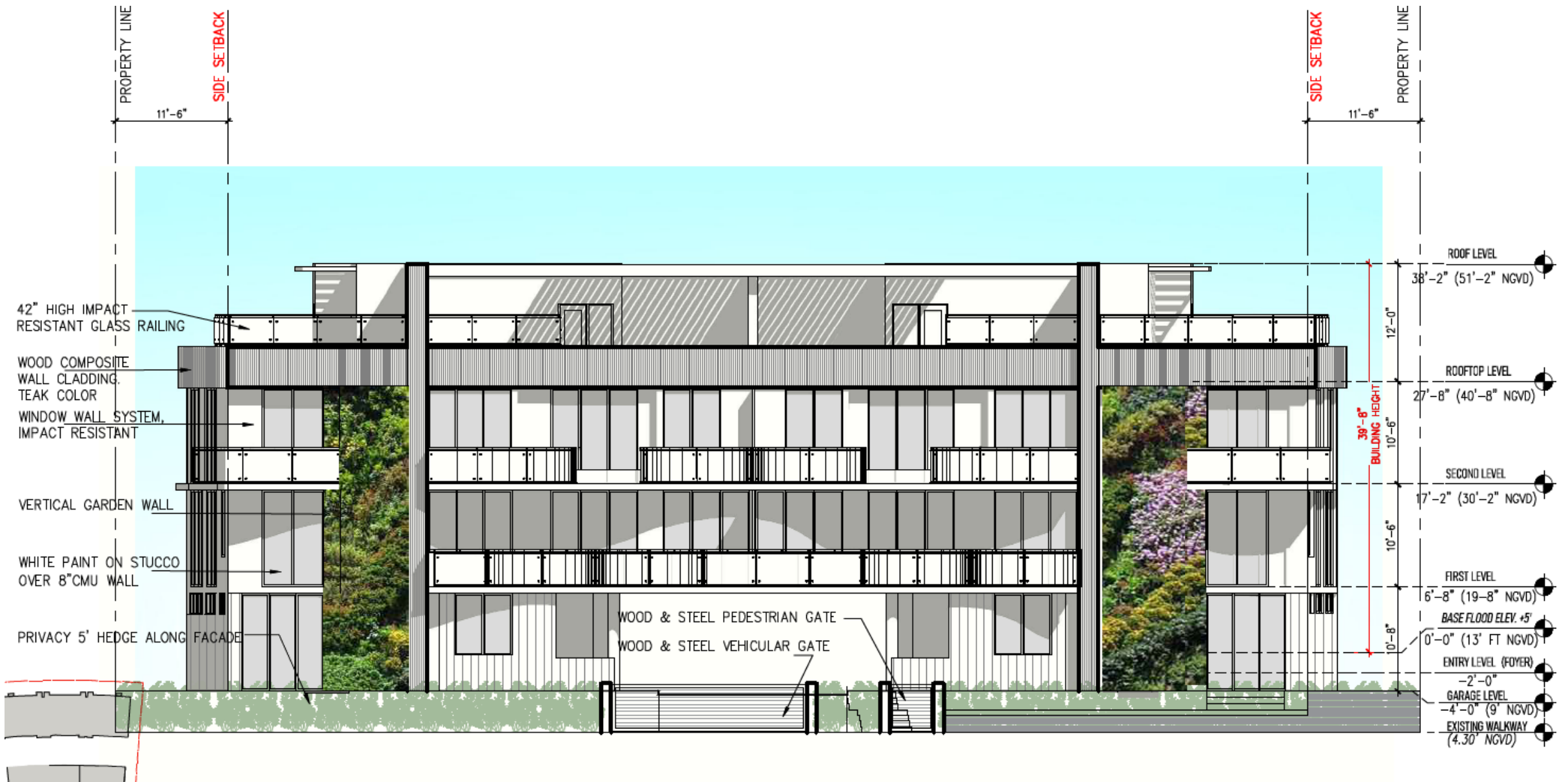
CALAIS DRIVE (SOUTH ELEVATION)
