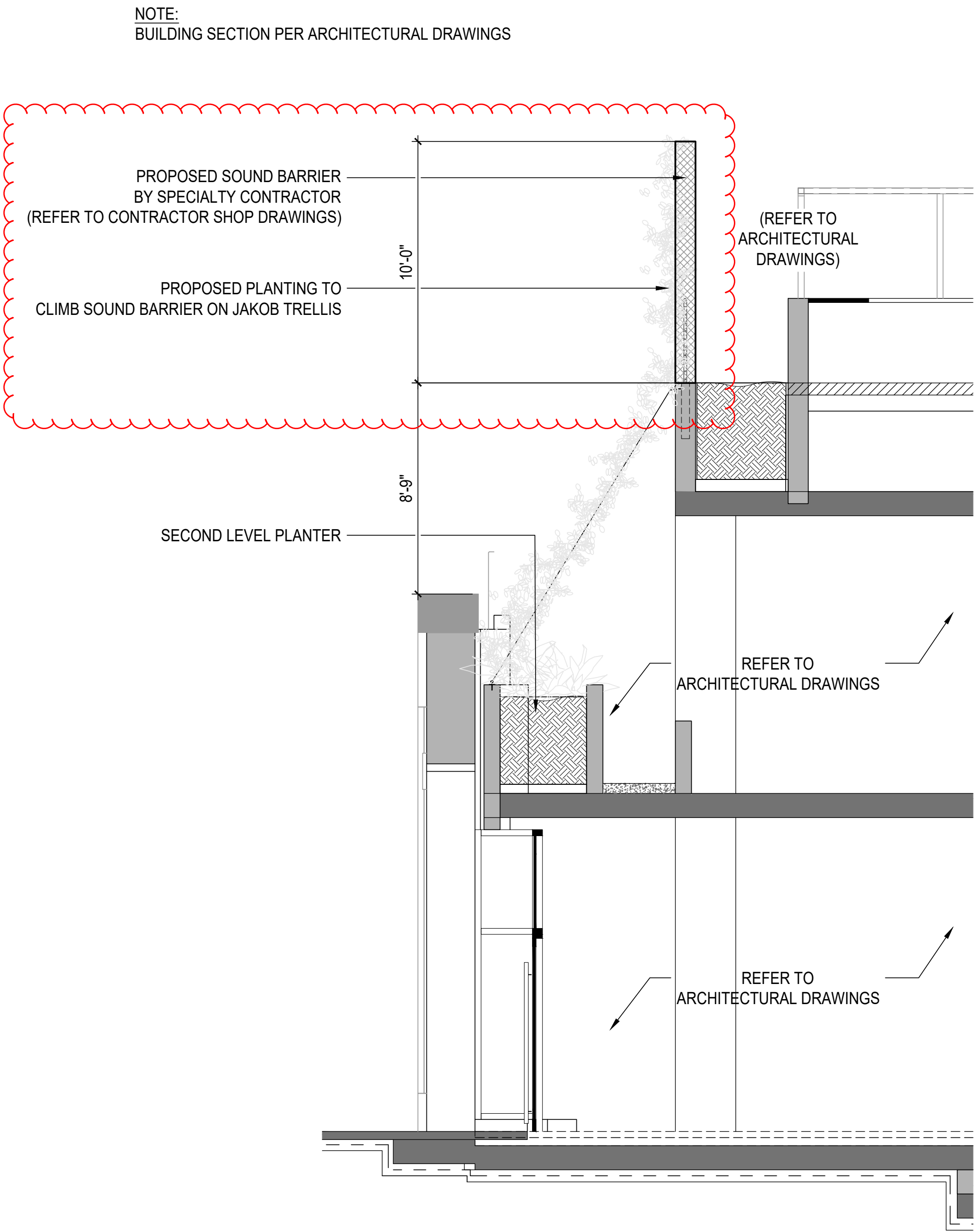
1 SOUND BARRIER SECTION AT POOL BAR Scale: 1/4" = 1'- 0"
