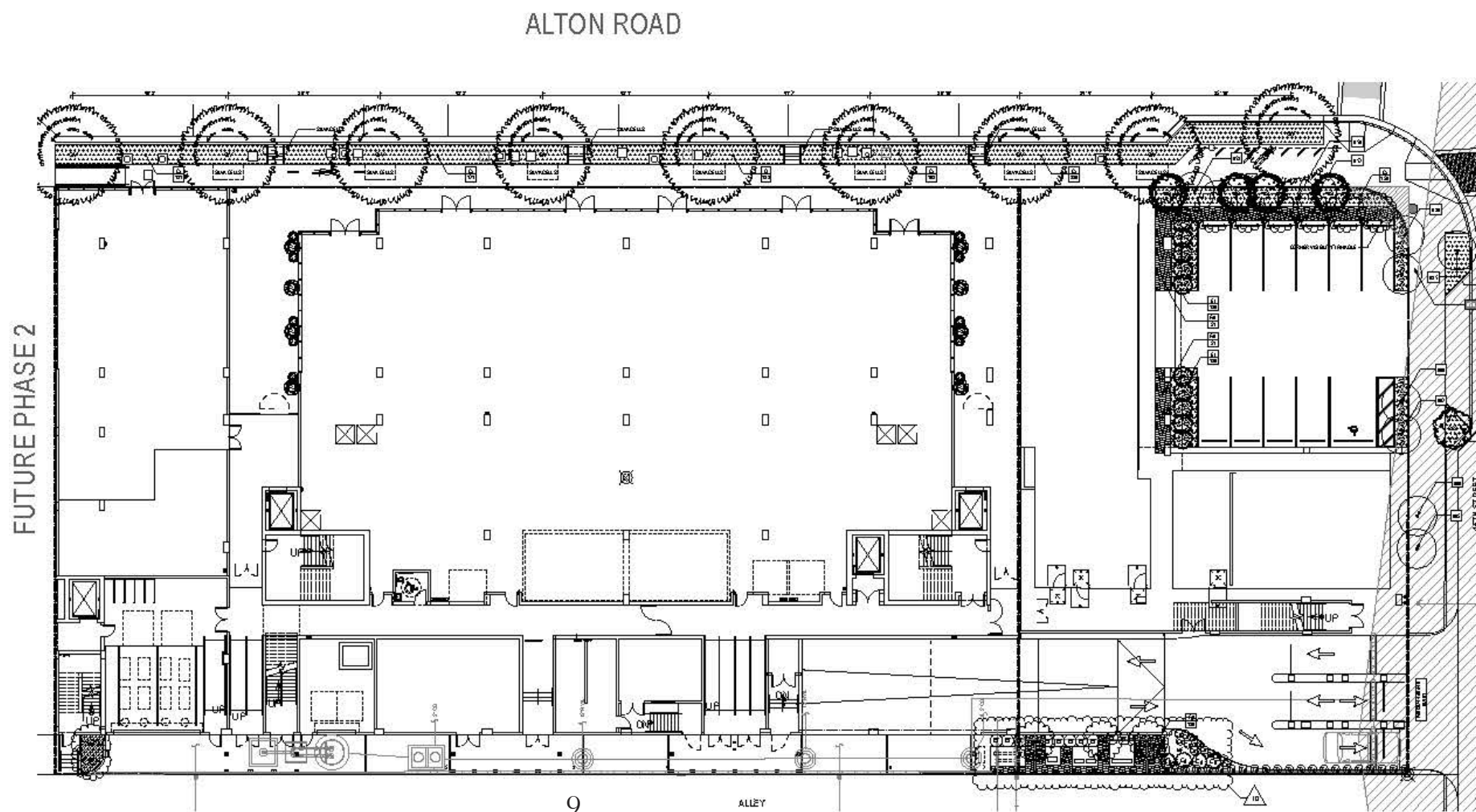
SITE PLANTING PLAN- PER PERMIT SUBMITTAL B1505070
