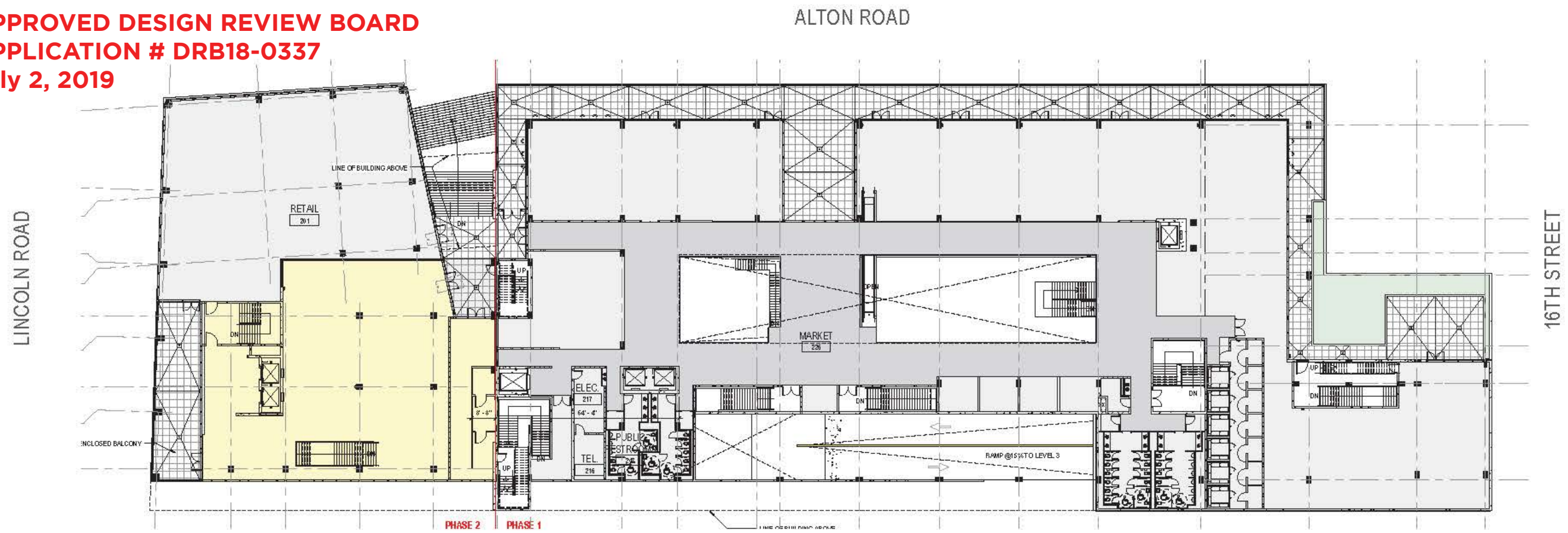
SECOND FLOOR PLAN - PREVIOUS DRB SUBMITTAL
