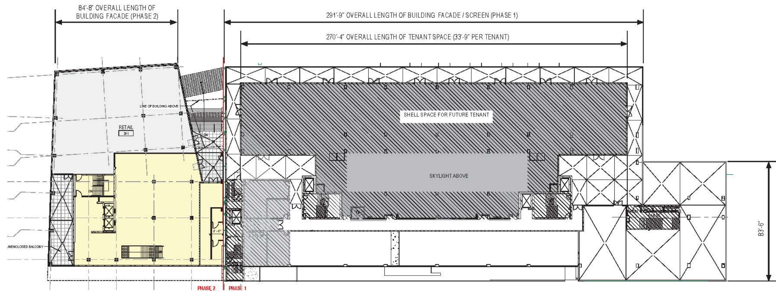
SECOND FLOOR PLAN - PREVIOUS DRB SUBMITTAL
