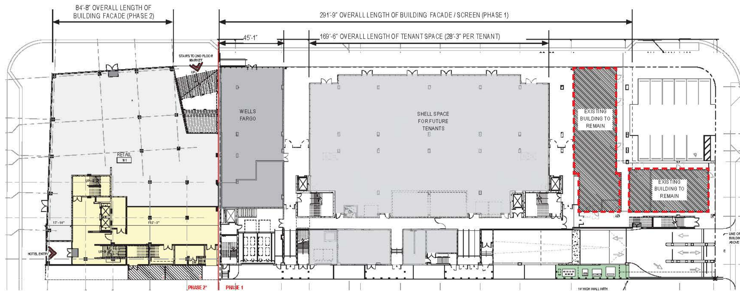
FIRST FLOOR PLAN- PER PERMIT SUBMITTAL B1505070
