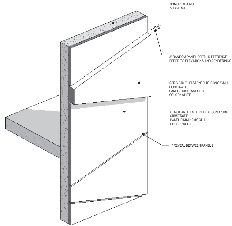
1 3D - EXTERIOR CLADDING DETAIL A3.02
