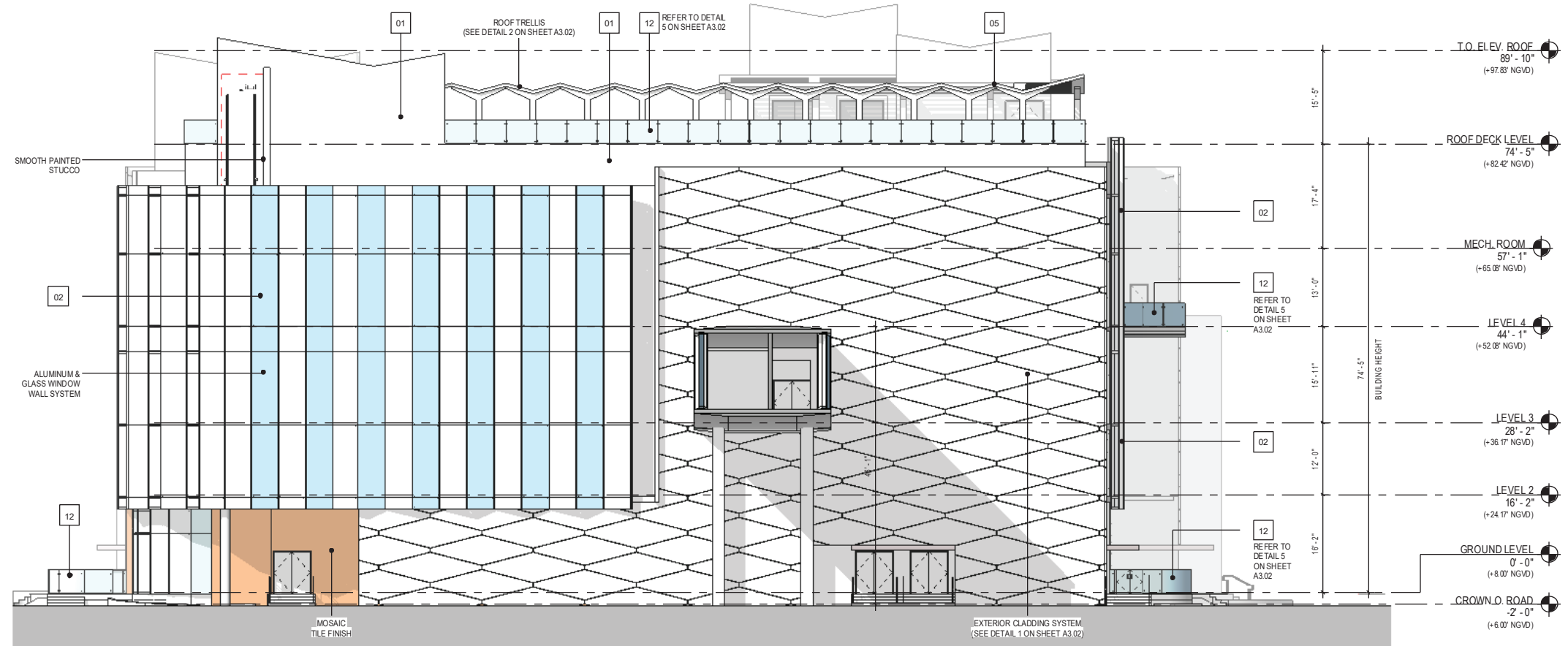
1 NORTH ELEVATION A3.01 3/32" = 1'-0"
