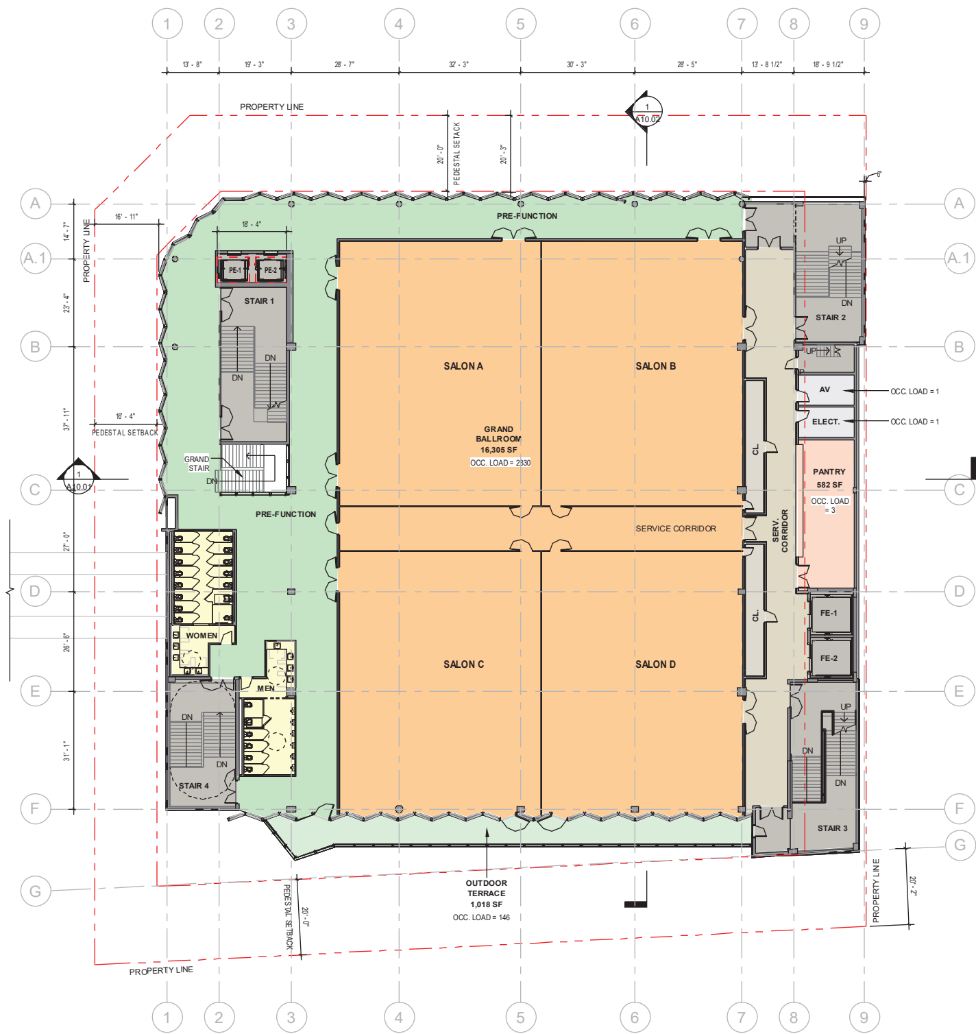
1 4TH LEVEL - FLOOR PLAN A1.04 1/16" = 1'-0"
