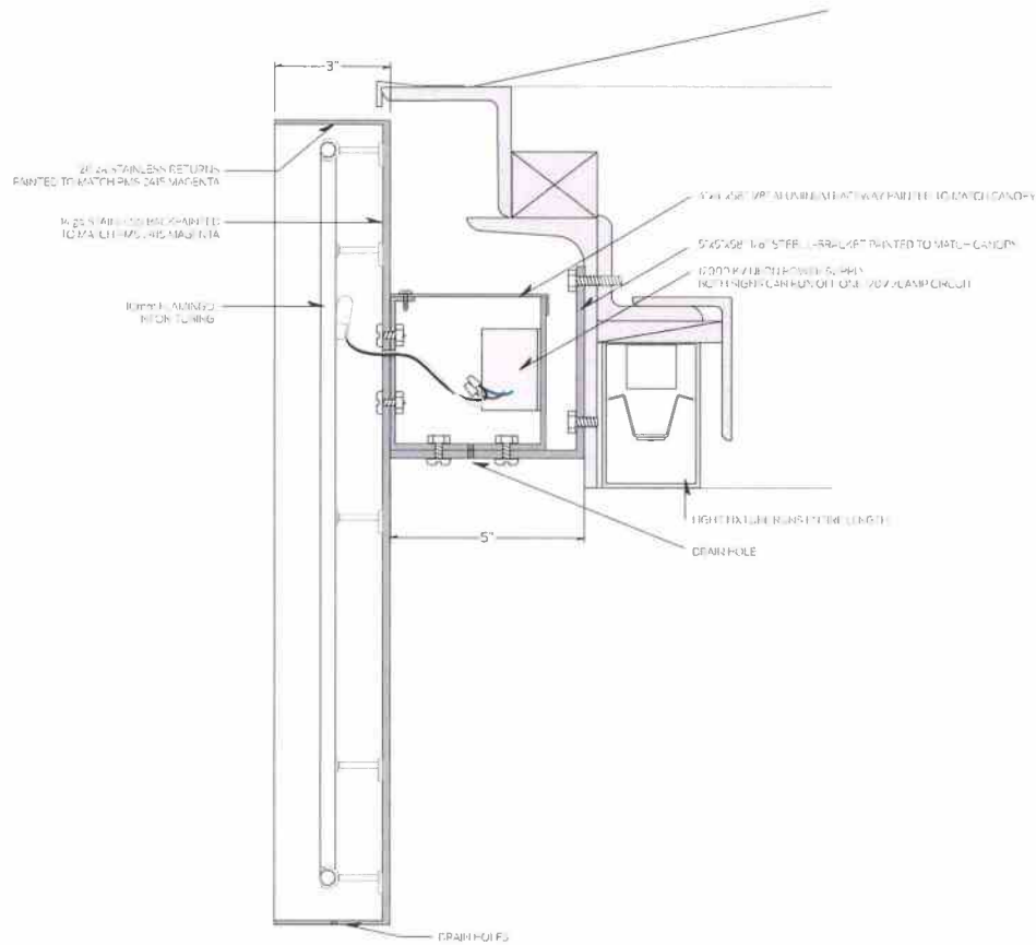
1 BUILDING ID B1.1 SECTION - FULL SCALE
