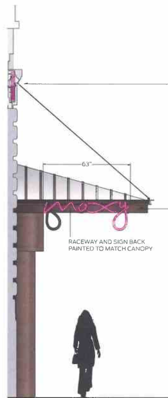
1 B1 & B1.1 SIDE ELEVATION - 1/10 SCALE
