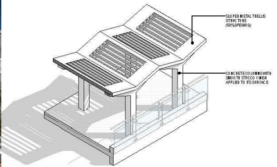
1 ENLARGED TRELLIS ROOF DETAIL A4.01
