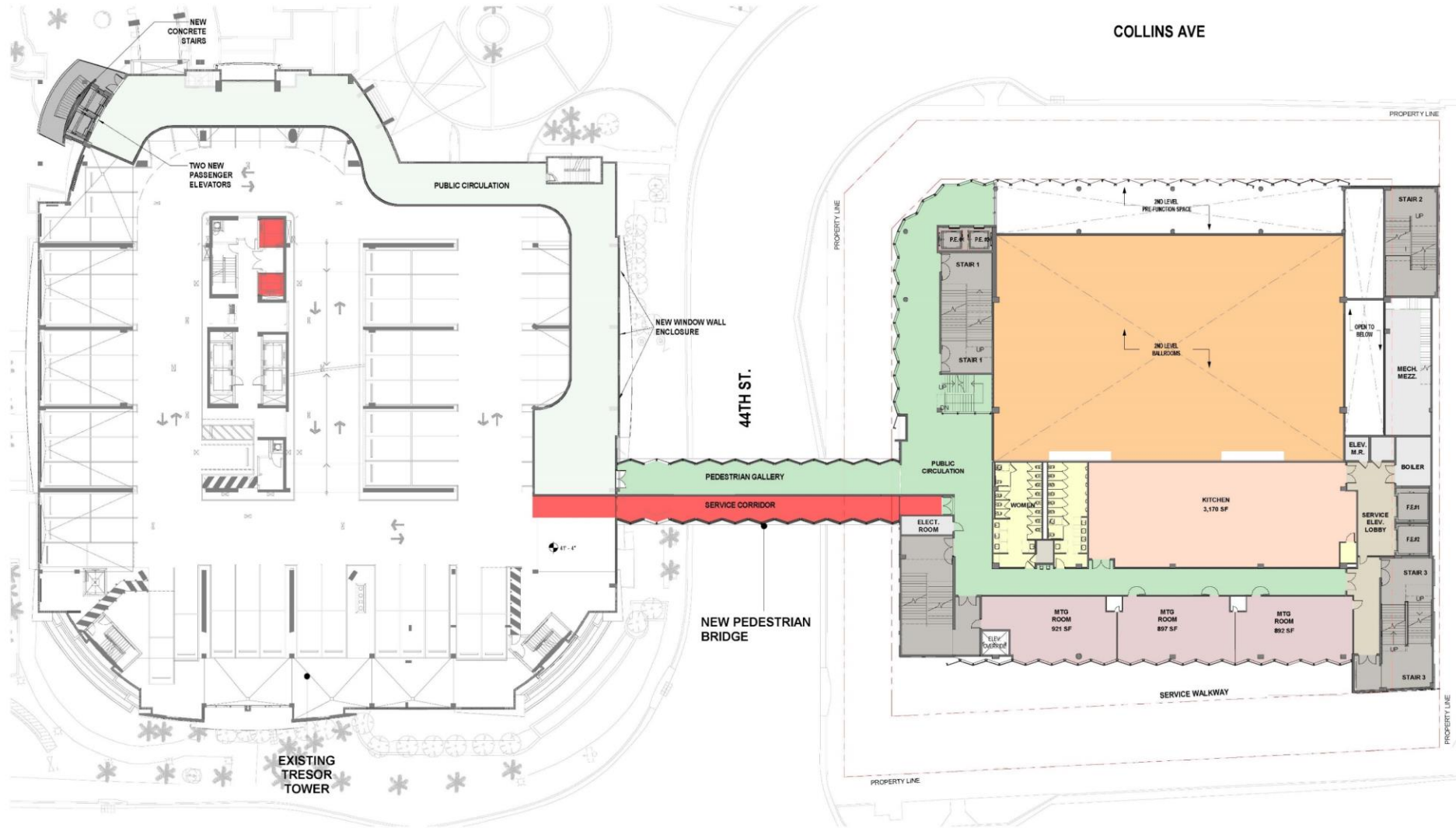
1 3RD LEVEL - OVERALL - FLOOR PLAN A1.03 1/16" = 1'-0"
