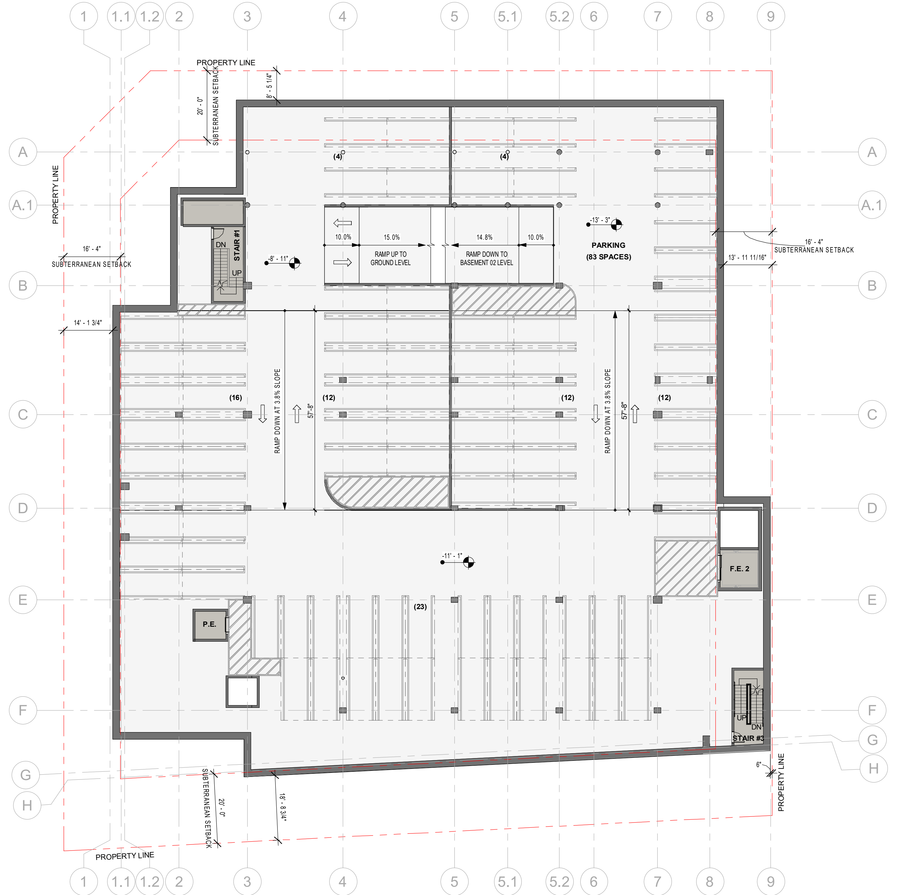
2 A1.00 BASEMENT LEVEL 1 - FLOOR PLAN 1/16" = 1'-0"
