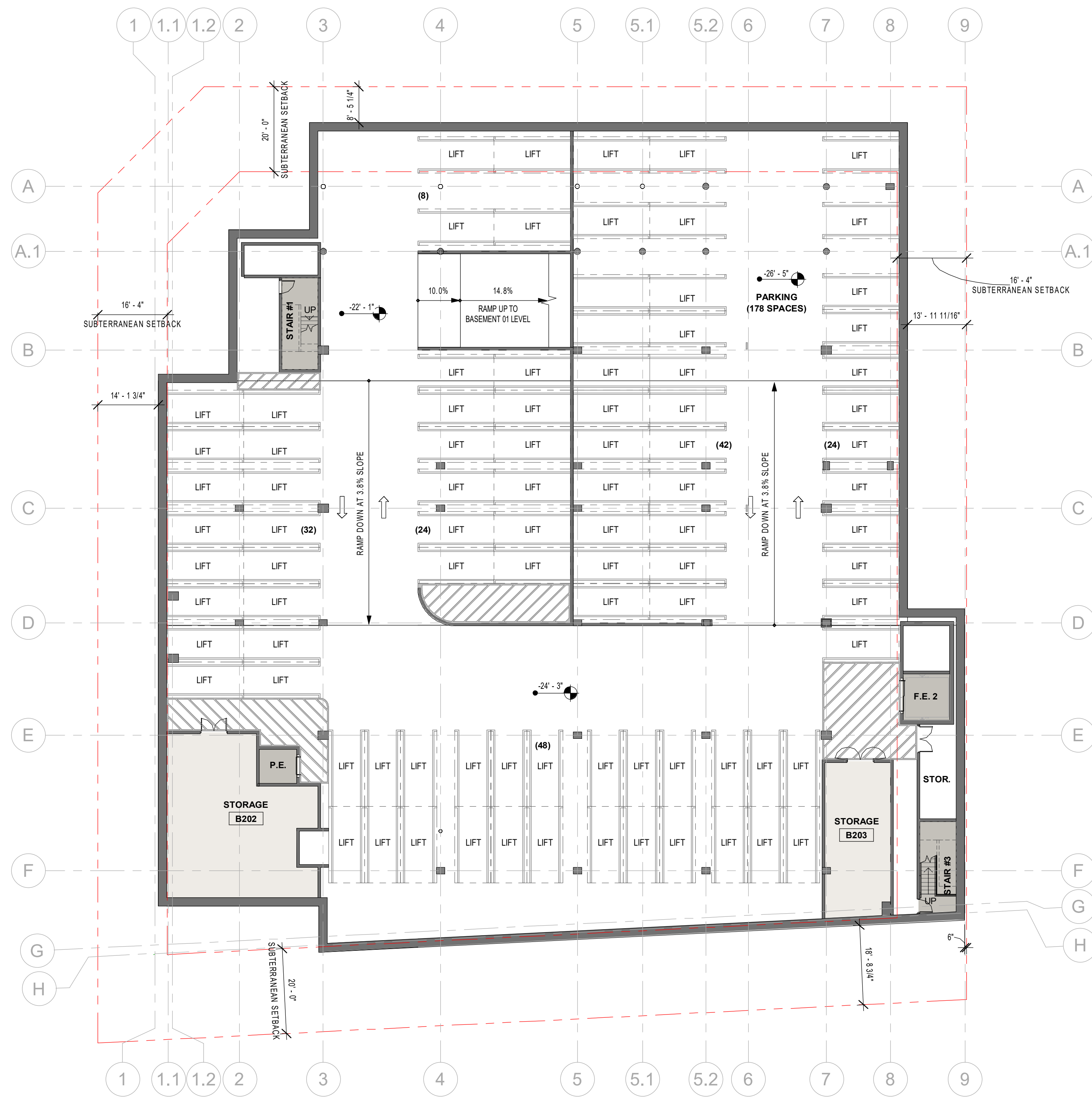
1 A1.00 BASEMENT LEVEL 2 - FLOOR PLAN 1/16" = 1'-0"
