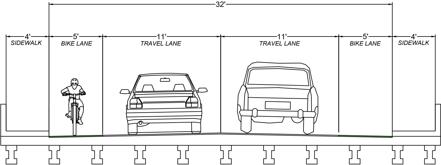
TYPICAL SECTION AT BRIDGES
