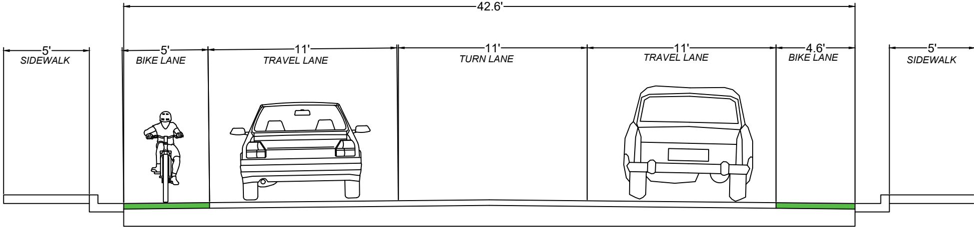
TYPICAL SECTION AT VENETIAN ISLANDS
