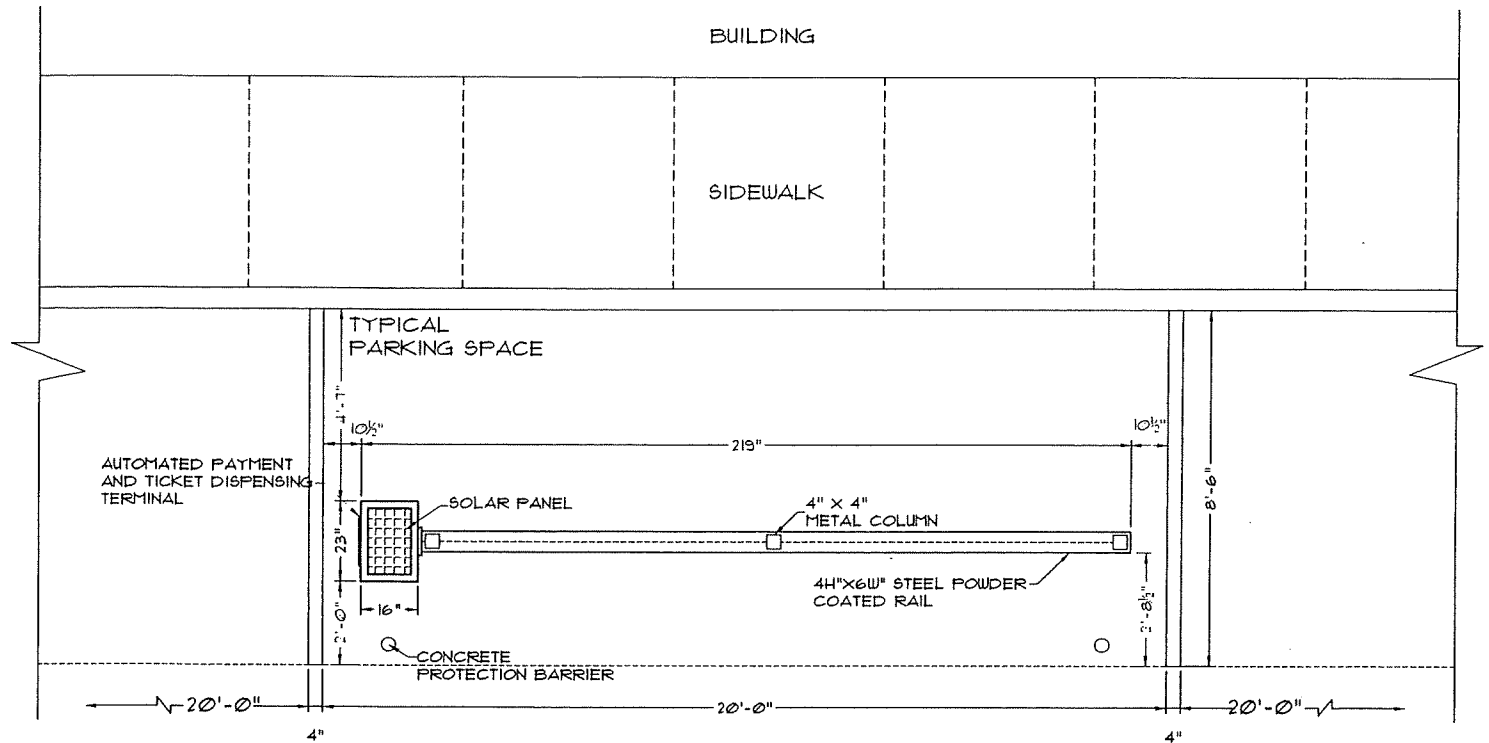
TYPICAL PARKING SPACE LAYOUT
