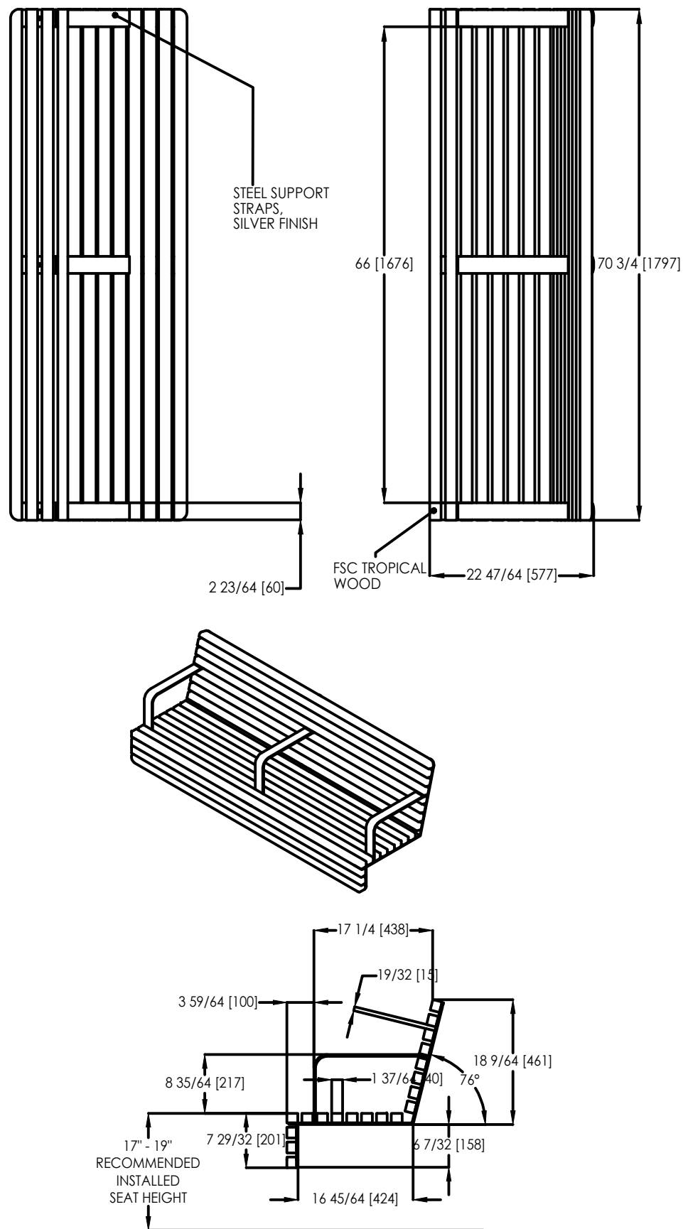
① TOP OF OOLITE WALL MOUNTED BENCH SCALE: N.T.S.
