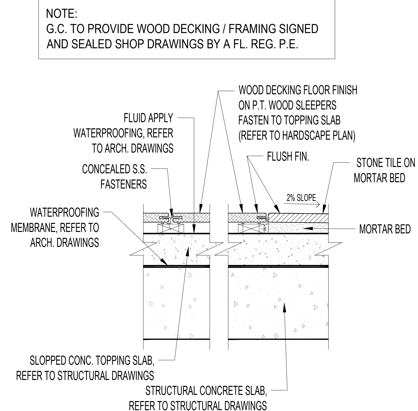
③ STONE MUDSET PAVER DETAIL SCALE: 3/4"=1'-0"
