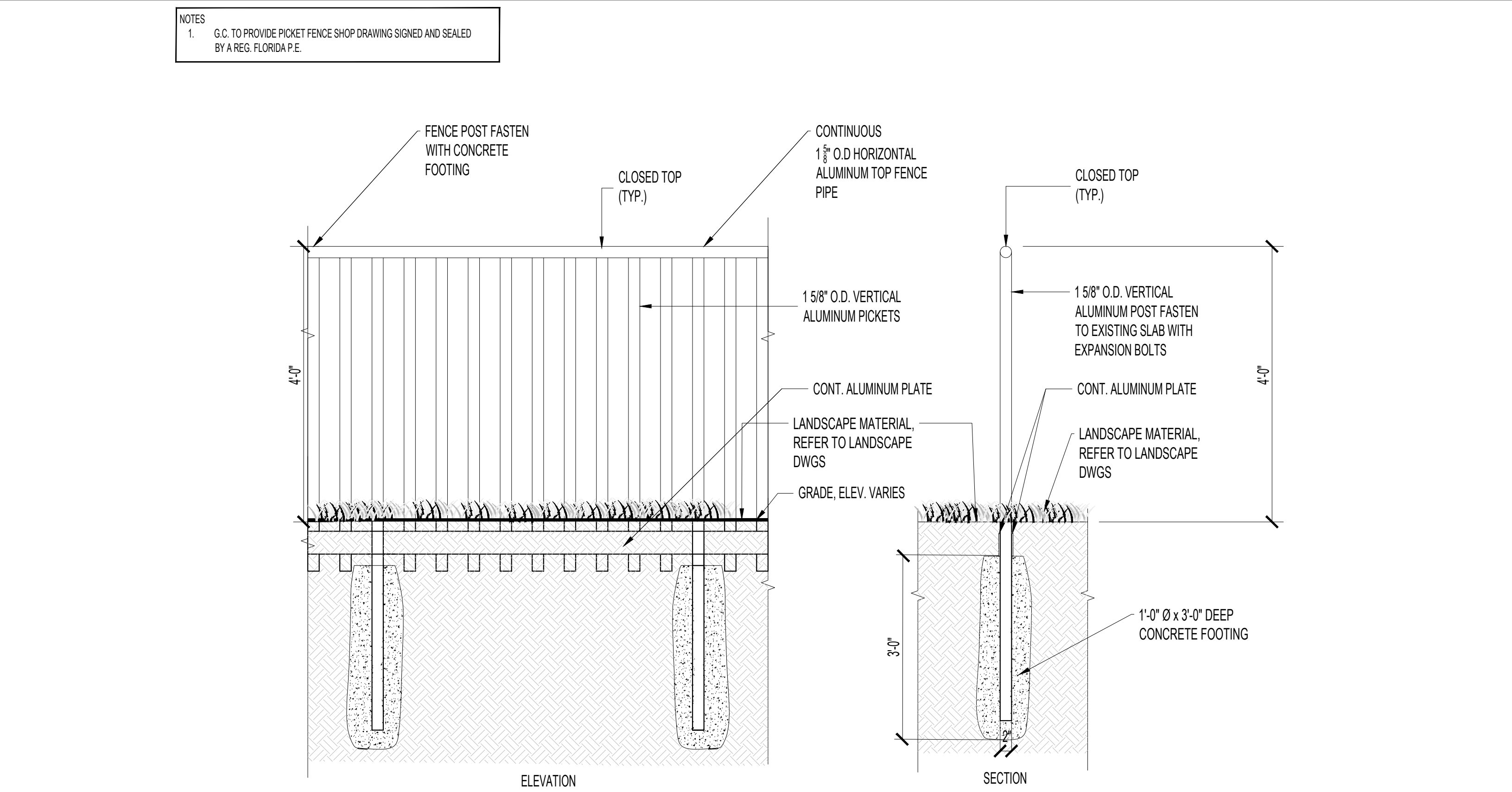
1 PLAYGROUND ALUMINUM FENCE WITH BRACING ON TOP SCALE: N.T.S.
