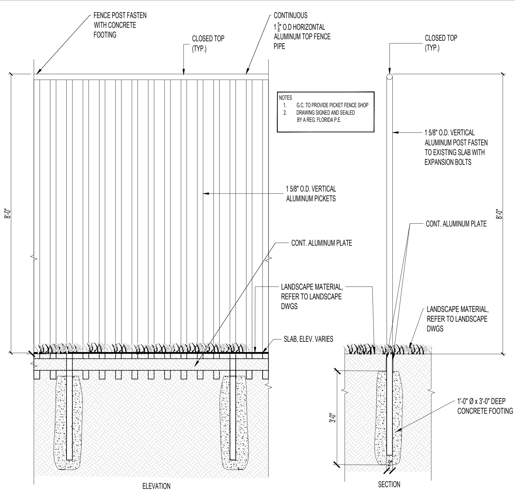
3 PRIVATE/PUBLIC ALUMINUM FENCE WITH BRACING ON TOP SCALE: N.T.S.
