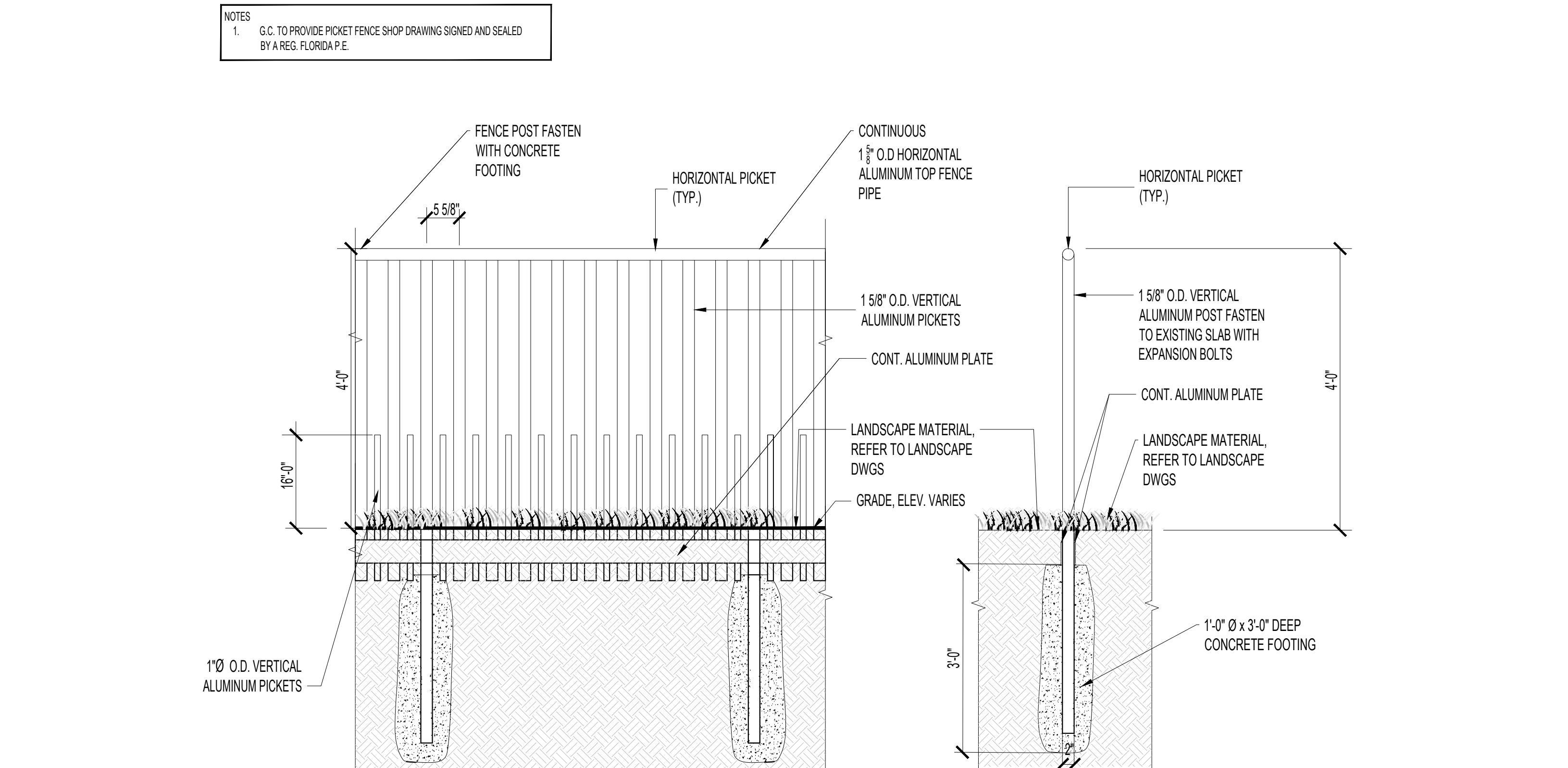
1 PLAYGROUND ALUMINUM FENCE WITH BRACING ON TOP SCALE: N.T.S.
