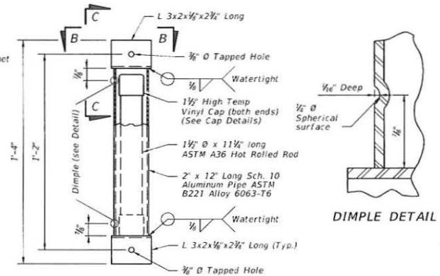
VIBRATION DAMPER ELEVATION
