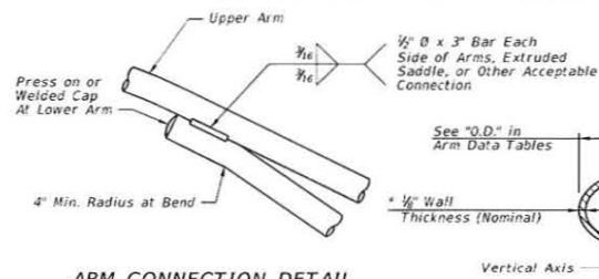
ARM CONNECTION DETAIL
