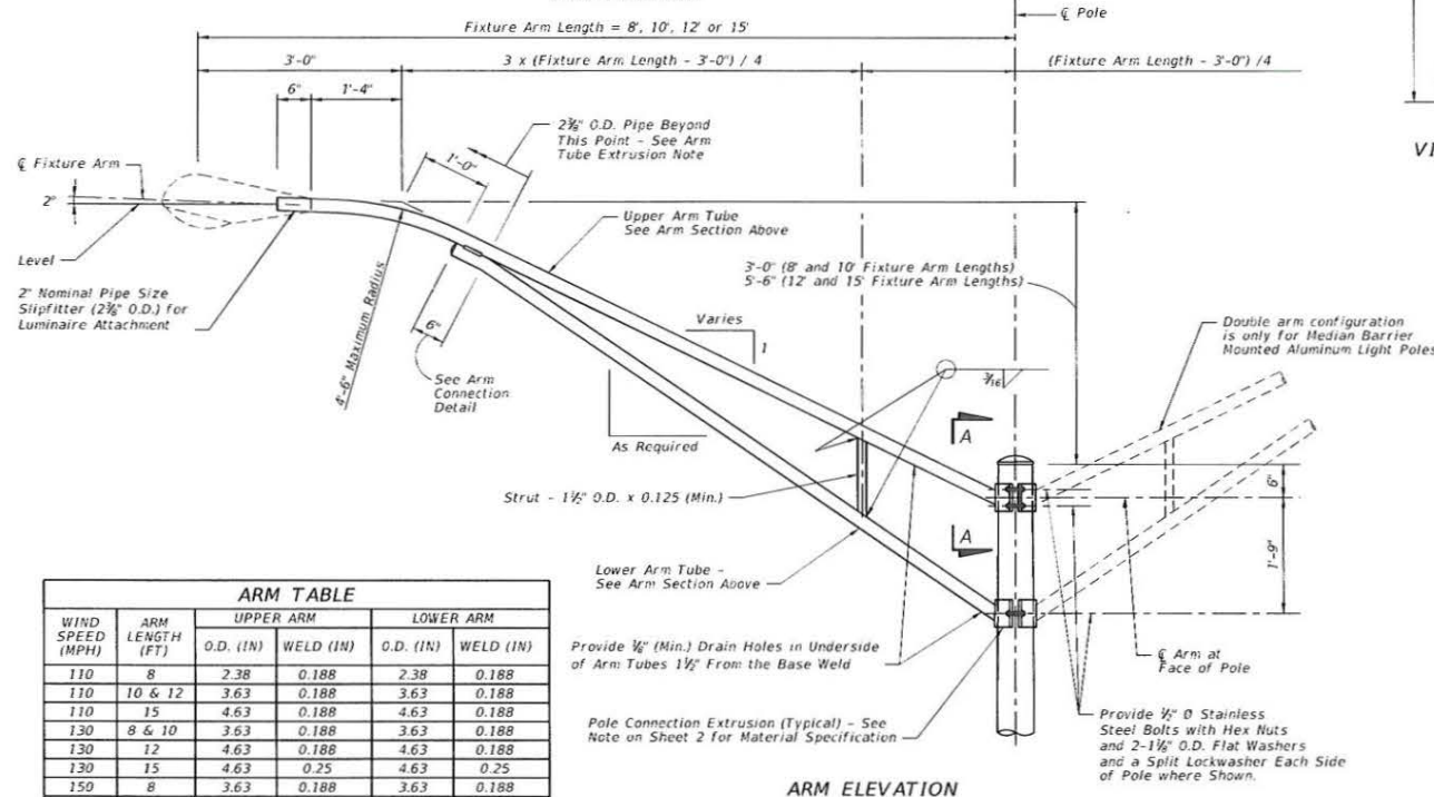
ARM ELEVATION
